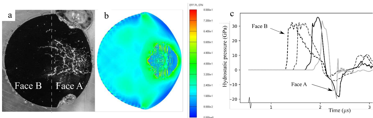
Figure 2: Comparison of (a) sectioned ball bearing (5.13g PE4), (b) the simulated effective plastic strain 2.5 \mu\text{s} after detonation, (c) Simulated pressure-time history inside the ball bearing for Face B (embedded) and face A (opposite to blast)
