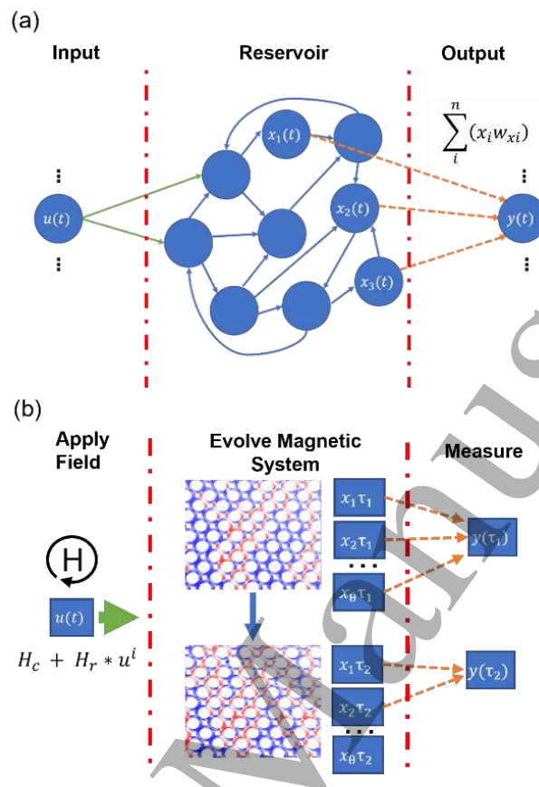
Figure 3: (a) The ESN approach to RC, showing the layered structure of the model: a fixed reservoir layer is provided with time-varying input via weighted connections. A linear output layer then provides a weighted sum of activities from nodes within the reservoir layer. (b) Our approach, where the ring array acts as a single dynamical node, into which time-multiplexed data is input using a rotating magnetic field, and output is extracted by measuring magnetic properties of the array at the end of each time-multiplexed input.
