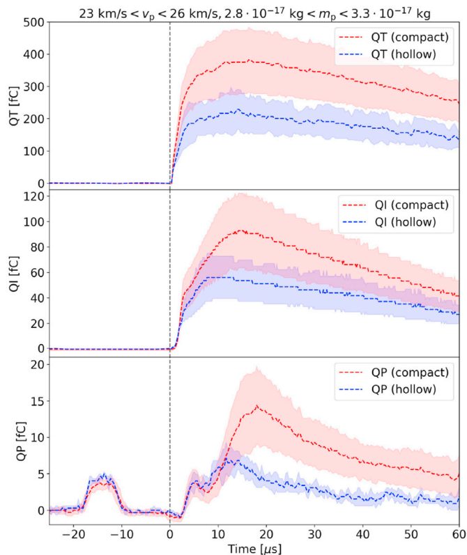
Fig. 16. Median QT, QI and QP signals from 108 to 11 IIT impacts of compact silicates from Batch II and hollow silicates, respectively, for a narrow range of dust masses m_p and impact velocities v_p . The filled areas around the signals indicate the spread of the data by showing the median absolute deviation of the different sets of signals that were used in the median. The impact time at t = 0 s is indicated by vertical dashed lines. Hollow particles of the same mass seem to generate less total impact charge.
