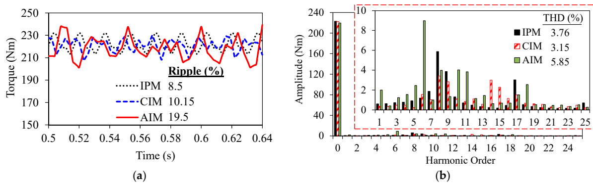
Figure 5. Comparison of the torque waveforms and their spectra. (a) Electromagnetic torque waveforms. (b) Harmonic spectra of torque.
