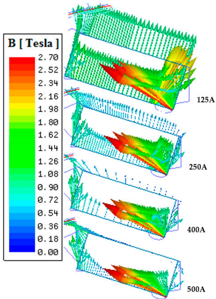
Figure 11. Flux density vectors of PMs for various electric loadings.
