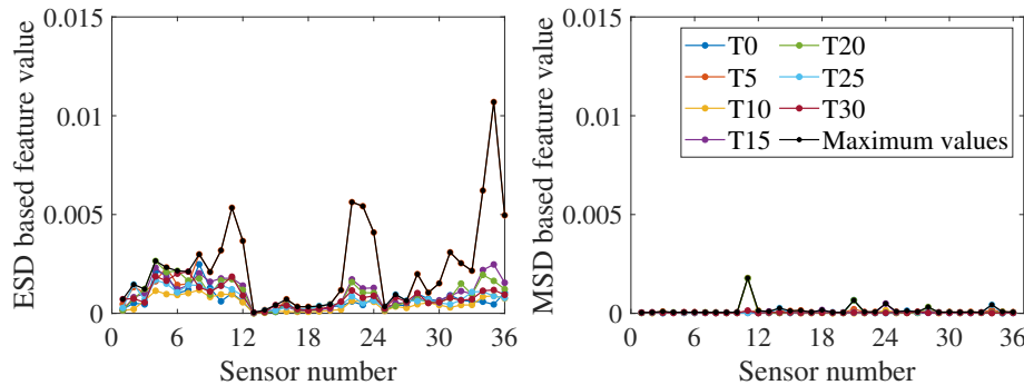
Figure 6. Feature-bagging results based on ESD (left) and MSD (right) for the normal condition. Seven controlled temperatures T0 – T30 and the maximum value among the features for seven different temperatures are shown by colour markers. ESD-based features refer to features obtained by the normalised approach with temperature labels. MSD-based features refer to features obtained by the linear approach without temperature labels.
