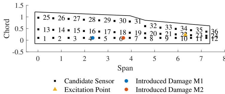
Figure 3. Labelled positions of experiment sets on the glider wing.
