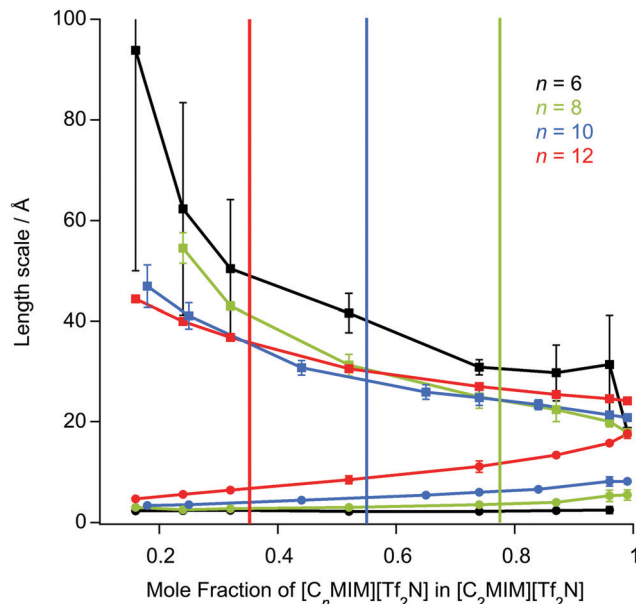
Fig. 7 The length scale parameters from the Teubner–Strey model for [C_n \text{mim}]_x [C_2 \text{mim}]_{1-x} [\text{Tf}_2 \text{N}] with data averaged for the [C_n \text{mim}]_x [C_2 \text{mim}-d_{11}]_{1-x} [\text{Tf}_2 \text{N}] and [C_n \text{mim}-d_{2n+7}]_x [C_2 \text{mim}]_{1-x} [\text{Tf}_2 \text{N}] contrasts ( n = 12, 10, 8 , and 6 ). The (upper) d -spacing data are squares whereas the (lower) correlation length data ( \zeta ) are circles. The green, blue and red, vertical lines represent the mole fraction corresponding to the crossing of the Lifshitz line for n = 12, 10 , and 8 , respectively.
