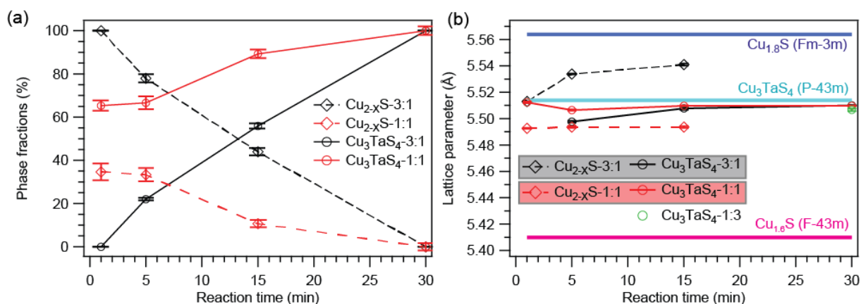
Figure 3. Analysis from Rietveld refinement profile. (a) Phase fractions of \text{Cu}_{2-x}\text{S} and \text{Cu}_3\text{TaS}_4 as a function of reaction time. (b) The calculated lattice parameters of \text{Cu}_{2-x}\text{S} and \text{Cu}_3\text{TaS}_4 compared with standard lattice parameters of \text{Cu}_{2-x}\text{S} ( x = 0.2 and 0.4 ), and \text{Cu}_3\text{TaS}_4 .
