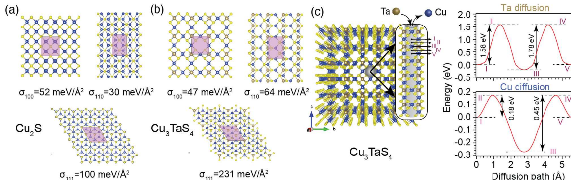
Figure 6. Schematics of low index surfaces of (a) \text{Cu}_2\text{S} and (b) \text{Cu}_3\text{TaS}_4 , from the top view, where light pink areas are 1 \times 1 unit cells, and \sigma is the surface formation energy. (c). Left panel demonstrates diffusion channels perpendicular to \{100\} planes inside \text{Cu}_3\text{TaS}_4 bulk, where the cylindrical grey shadow, in the inset, schematically shows the Ta and Cu diffusion path. Right panels are the diffusion energy barriers for Ta and Cu along the diffusion channel, where the Roman numerals are used to link the crystal coordinates to their corresponding points along the diffusion path.
