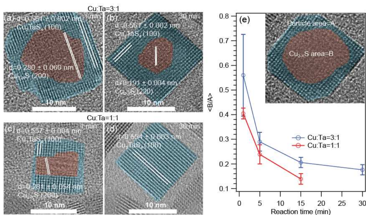
Figure 5. High resolution transmission electron microscopy (HRTEM) images of the core-shell type \text{Cu}_{2-x}\text{S} - \text{Cu}_3\text{TaS}_4 NCs. (a-b) NCs of 1 min, and 30 min reaction for Cu:Ta = 3:1. (c-d) NCs of 1 min, and 30 min reaction for Cu:Ta = 1:1. The HRTEM images for Cu:Ta = 1:3 reactions are shown in Figure S6 . (e) The average of core to particle area ratio as a function of reaction time for Cu:Ta = 3:1 and Cu:Ta = 1:1. Inset figure is schematic presentation of the core-shell type \text{Cu}_{1.8}\text{S} - \text{Cu}_3\text{TaS}_4 NCs.
