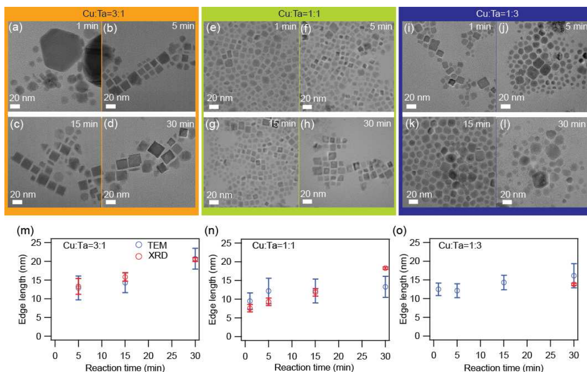
Figure 4. TEM images of the synthesized NCs. (a-d) Cu:Ta = 3:1, (e-h) Cu:Ta = 1:1, and (i-l) Cu:Ta = 1:3 for different reaction times: 1 min, 5 min, 15 min, and 30 min. The scale bar is 20 nm. The average edge length as a function of reaction time for (m) Cu:Ta = 3:1, (n) Cu:Ta = 1:1, and (o) Cu:Ta = 1:3. The error bars indicate the size distribution. The average size calculated from TEM images are shown by blue solid circles and the size calculated from the XRD peaks after Rietveld refinement is shown by open black circles. The size distribution histograms are shown in Figure S5 .
