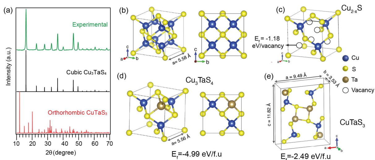
Figure 1. (a) PXRD pattern of the synthesized nanocrystals (green line) (after 30 min reaction) compared with standard orthorhombic phase \text{CuTaS}_3 (red line) and cubic phase \text{Cu}_3\text{TaS}_4 (black line). Ball and stick model of (b) \text{Cu}_2\text{S} , (c) \text{Cu}_{2-x}\text{S} , (d) cubic \text{Cu}_3\text{TaS}_4 , and (e) orthorhombic \text{CuTaS}_3 , where blue, yellow, and brown balls represent Cu, S, and Ta atoms, respectively. E_f denotes the formation energies of vacancies in (c), and bulk crystal in (d) and (e).
