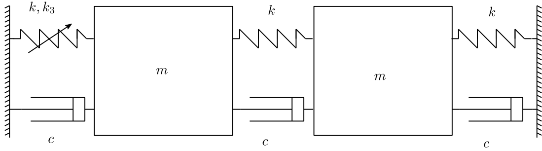
Fig. 2. Schematic of the two-DOF system used in this paper.
