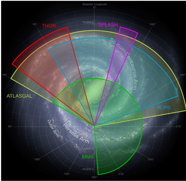
Figure 1. Image depicting the Galactic longitude coverages for the Galactic plane surveys that are utilized in this study (courtesy of NASA/JPL-Caltech/R. Hurt (SSC/Caltech)). The approximate coverage of each survey is shown along with each survey’s corresponding name. The length of each sector is arbitrary.
