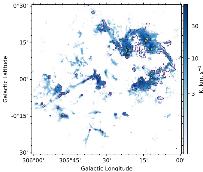
Fig. 3. ^{13}\text{CO}(3-2) moment-0 map of the G305 region. Overlaid are the contours of ATLASGAL corresponding to intensities 0.6, 1, and 3 Jy/beam.
