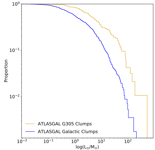
Fig. 10. CDF of L_{\text{clumps}}/M_{\text{clumps}} in G305 compared to that of the ATLASGAL Galactic clumps.
