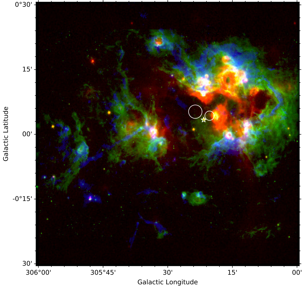
Fig. 1. Three-color image (green = Spitzer -IRAC4 8 \mu\text{m} , red = Midcourse Space Experiment (MSX) 21.3 \mu\text{m} , blue = LAsMA ( ^{13}\text{CO}(3-2) moment-0)) of the G305 star-forming complex. The 21.3 \mu\text{m} emission is dominated by hot dust in the HII region. The colder gas is traced by the ^{13}\text{CO}(3-2) line emission. The interface between the ionized and molecular gas appears as a blend of green (strong 8 \mu\text{m} emission from PAHs), blue (colder molecular gas), and occasionally red (interfaces very close to HII regions). The positions of the Danks 1 and 2 clusters are given by the smaller and the larger white circles, respectively, and WR48a is shown as a white star.
