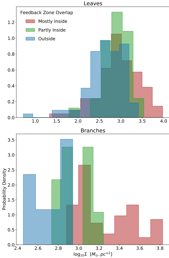
Fig. 8. Histogram of the probability density of surface mass densities of leaves ( top ) and branches ( bottom ) based on their overlap with the feedback zone defined using an 8 \mu\text{m} threshold of 100 \text{ MJy sr}^{-1} .
