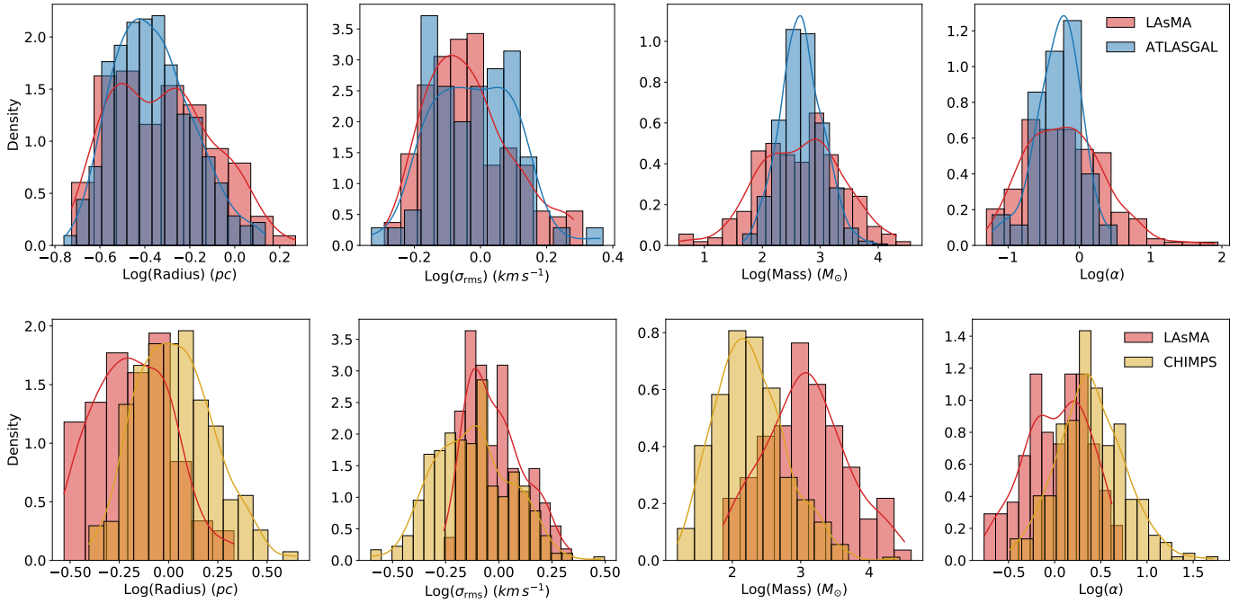
Fig. 9. Comparison of properties of LAsMA clumps in G305 with a Galactic sample derived from ATLASGAL ( top panel ) and CHIMPS ( bottom panel ) surveys. The solid lines overlaid in matching colors show the KDE of the distribution of the corresponding properties.
