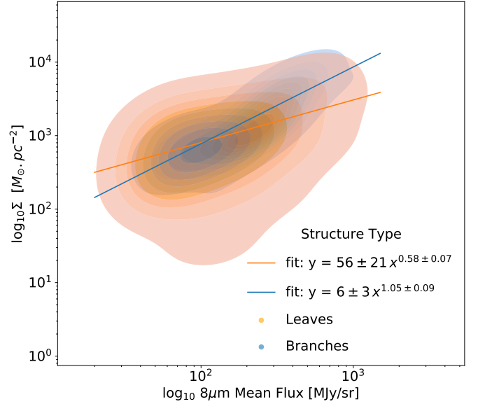
Fig. 7. Surface mass density of clumps in G305 as a function of 8\ \mu\text{m} flux. The orange and blue lines show the results of a power law fit to these quantities for leaves and branches respectively.
