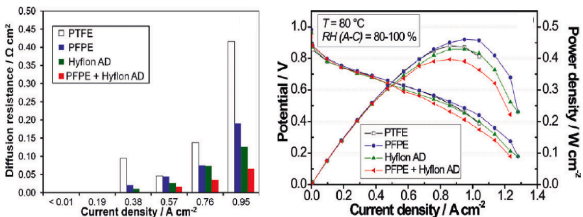
Fig. 20. The diffusion resistance of the GDLs with MPL different compositions ( 60^\circ\text{C} , 80–100% RH). (Right) Polarisation curve of MEAs with the differing MPL compositions ( 80^\circ\text{C} and 80–100% RH). Reproduced from Fuel Cells with the permission of John Wiley and Sons [189].
