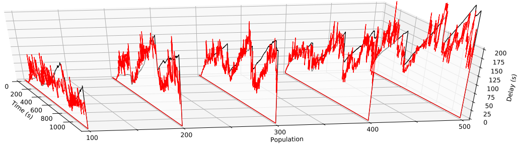
Regression emulator predicts delays - Experiment 2: Population=100 to 500, Step ahead = 15
