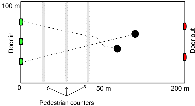
Fig. 4: The StationSim model; adapted from Malleon et al. (2020)
