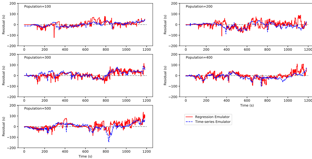
Fig. 10: Comparison between the prediction errors from regression versus time-series emulators
