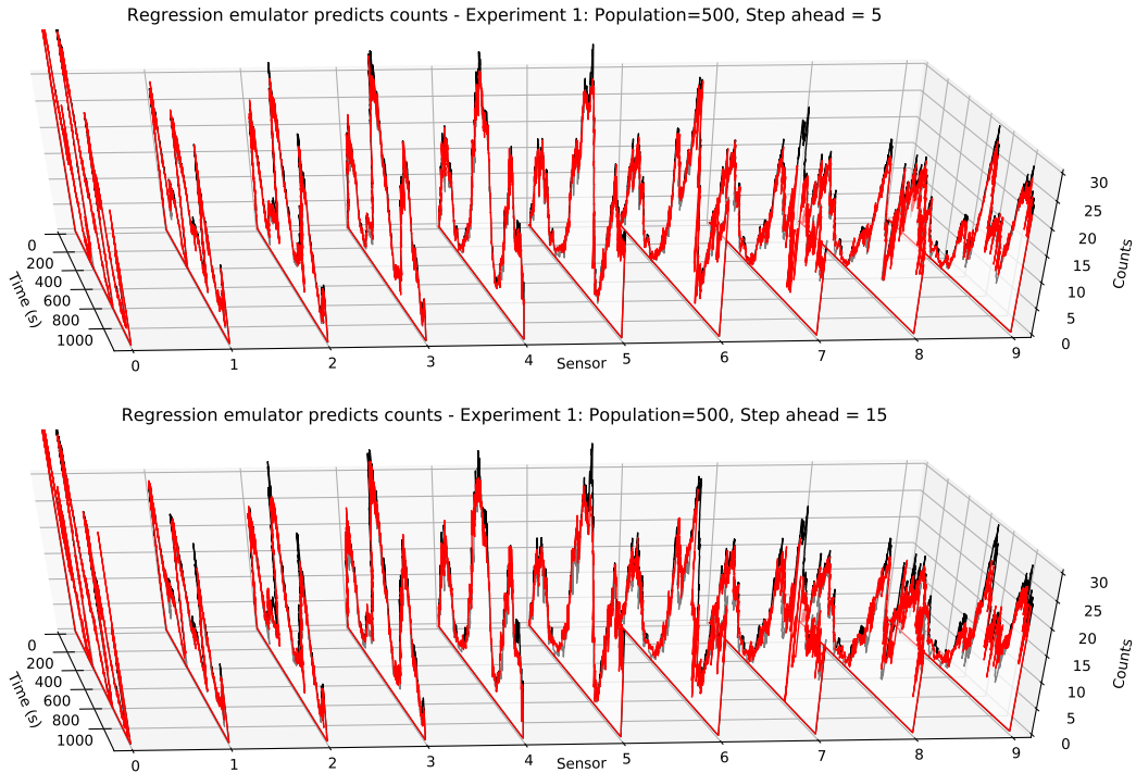
Fig. 6: Prediction of pedestrian counts at each sensor using the the regression emulator. Red line: Predicted counts, Black line: Synthetic real-time counts
