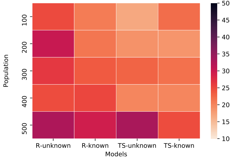
Fig. 14: Comparison of the prediction results for delay. R-unknown: Regression emulator predicts unknown population, R-known: Regression emulator predict known population, TS-unknown: Time-series emulator predicts unknown population, TS-known: Time-series emulator predicts known population
