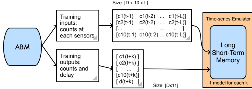
Fig. 3: A time-series emulator of Agent-Based Models using Long Short-term Memory
