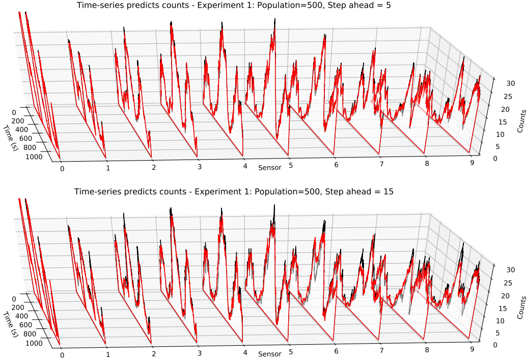
Fig. 7: Prediction of pedestrian counts at each sensor using the time-series emulator. Red line: Predicted counts, Black line: Synthetic real-time counts
