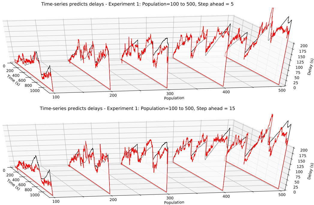
Fig. 9: Prediction of delays using the time-series emulator. Red line: Predicted delay, Black line: Synthetic real-time delay
