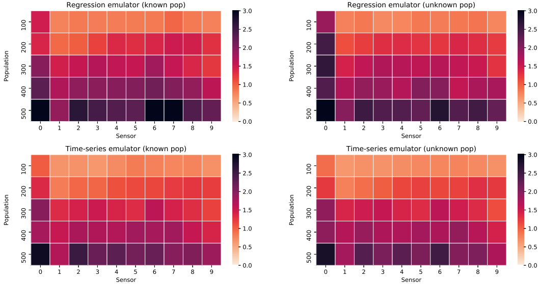
Fig. 11: Comparison of the prediction results for aggregated pedestrian counts at each sensor
