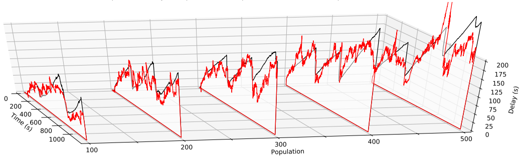
Fig. 13: Experiment 2: Prediction of delays using the time-series emulator. Red line: Predicted delay, Black line: Synthetic real-time delay
