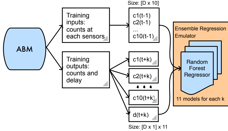
Fig. 2: A regression emulator of Agent-Based Models using Random Forest Regression
