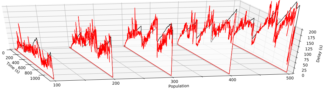
Fig. 8: Prediction of delays using the the regression emulator. Red line: Predicted delay, Black line: Synthetic real-time delay
