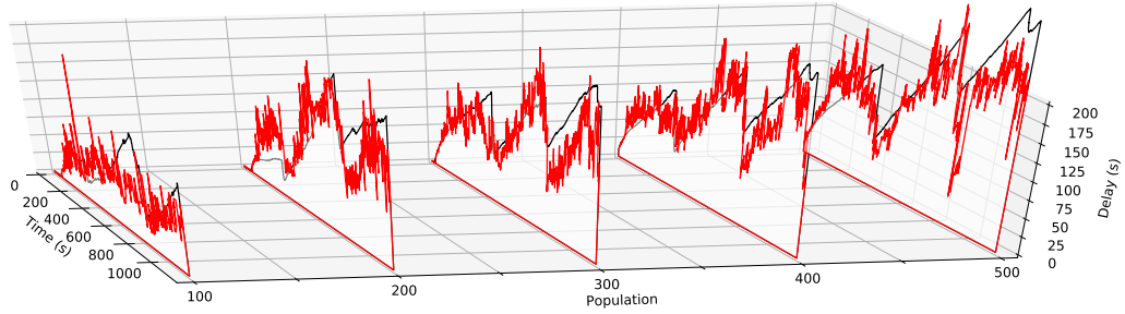
Fig. 12: Experiment 2: Prediction of delays using the the regression emulator. Red line: Predicted delay, Black line: Synthetic real-time delay
