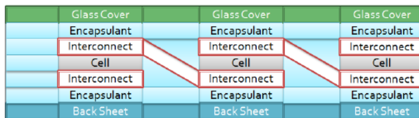
Figure 9. Cross section of a PV module [67].
