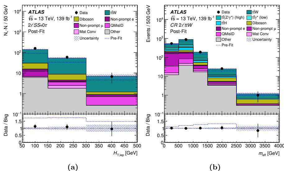
Figure 6. (a) Comparison between data and the background prediction for the distribution of the scalar sum of the lepton p_T ( H_{T, \text{lep}} ) in the 2\ell\text{SS}+0\tau channel, obtained by subtracting the corresponding distributions for events with positive and negative total charge. In (b) the comparison is performed for the m_{\text{eff}} distribution in the 2\ell\text{ttW} CR without splitting according to total charge. The background contributions after the likelihood fit to data (“Post-Fit”) under the background-only hypothesis are shown as filled histograms. The total background prediction before the likelihood fit to data (“Pre-Fit”) is shown as a dashed blue histogram in the upper panel. The ratio of the data to the background (“Bkg”) prediction is shown in the lower panel, separately for post-fit background (black points) and pre-fit background (dashed blue line). The size of the combined statistical and systematic uncertainty in the background prediction is indicated by the blue hatched band. The last bin in each figure contains the overflow.
