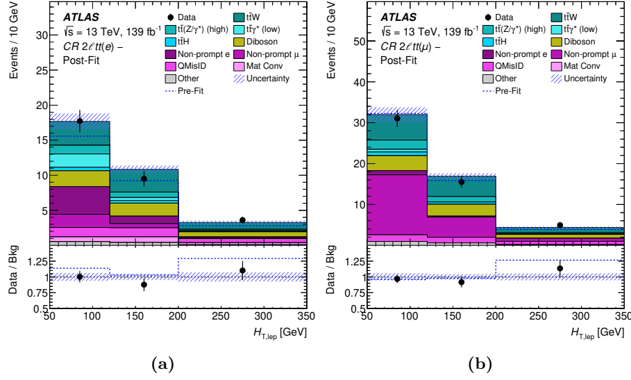
Figure 9. Comparison between data and the background prediction for the distribution of the scalar sum of the lepton p_T ( H_{T, \text{lep}} ) in (a) the 2\ell tt(e) - CR and (b) the 2\ell tt(\mu) - CR. The background contributions after the likelihood fit to data (“Post-Fit”) under the background-only hypothesis are shown as filled histograms. The total background prediction before the likelihood fit to data (“Pre-Fit”) is shown as a dashed blue histogram in the upper panel. The ratio of the data to the background (“Bkg”) prediction is shown in the lower panel, separately for post-fit background (black points) and pre-fit background (dashed blue line). The size of the combined statistical and systematic uncertainty in the background prediction is indicated by the blue hatched band. The last bin in each figure contains the overflow.
