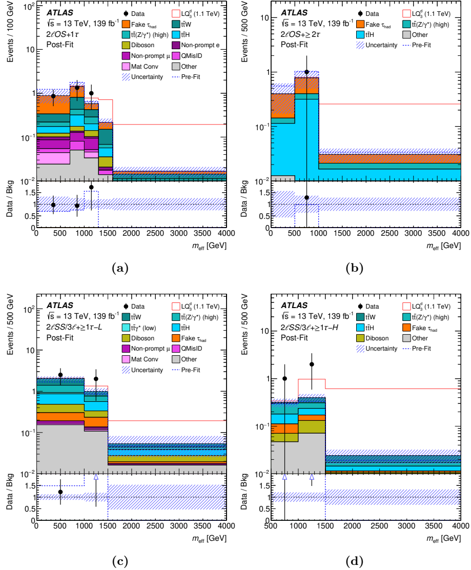
Figure 13. Comparison between data and prediction for the m_{\text{eff}} distribution used in different signal region categories of the 2\ell OS + \geq 1\tau and 2\ell SS/3\ell + \geq 1\tau channels: (a) 2\ell OS + 1\tau , (b) 2\ell OS + \geq 2\tau , (c) 2\ell SS/3\ell + \geq 1\tau-L , and (d) 2\ell SS/3\ell + \geq 1\tau-H . The background contributions after the likelihood fit to data (“Post-Fit”) under the background-only hypothesis are shown as filled histograms. For illustrative purposes, the expected signal for m_{LQ_3^d} = 1.1 TeV and \mathcal{B} = 1 is shown as unfilled red histogram added to the post-fit background. The total background prediction before the likelihood fit to data (“Pre-Fit”) is shown as a dashed blue histogram in the upper panel. The ratio of the data to the background (“Bkg”) prediction is shown in the lower panel, separately for post-fit background (black points) and pre-fit background (dashed blue line). The size of the combined statistical and systematic uncertainty in the background prediction is indicated by the blue hatched band. The blue triangles indicate points that are outside the vertical range of the figure. The last bin in each figure contains the overflow.
