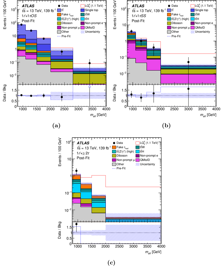
Figure 12. Comparison between data and prediction for the m_{\text{eff}} distribution used in different signal region categories of the 1\ell + \geq 1\tau channel: (a) 1\ell + 1\tau_{\text{OS}} , (b) 1\ell + 1\tau_{\text{SS}} , and (c) 1\ell + \geq 2\tau . The background contributions after the likelihood fit to data (“Post-Fit”) under the background-only hypothesis are shown as filled histograms. For illustrative purposes, the expected signal for m_{LQ_3^d} = 1.1 TeV and \mathcal{B} = 1 is shown as a unfilled red histogram added to the post-fit background. The total background prediction before the likelihood fit to data (“Pre-Fit”) is shown as a dashed blue histogram in the upper panel. The ratio of the data to the background (“Bkg”) prediction is shown in the lower panel, separately for post-fit background (black points) and pre-fit background (dashed blue line). The size of the combined statistical and systematic uncertainty in the background prediction is indicated by the blue hatched band. The blue triangles indicate points that are outside the vertical range of the figure. The last bin in each figure contains the overflow.
