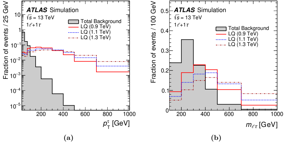
Figure 1. Comparison of the distribution of (a) the p_{\text{T}} of the \tau_{\text{had}} candidate ( p_{\text{T}}^\tau ), and (b) the invariant mass of the light lepton and the \tau_{\text{had}} candidate ( m_{\ell\tau} ), between the total background (shaded histogram) and the LQ signal for different mass values. The selection used corresponds to events in the 1\ell+1\tau event category (a) after the preselection requirements, and (b) after applying the additional requirement of p_{\text{T}}^\tau > 150 GeV. The last bin in each distribution contains the overflow.
