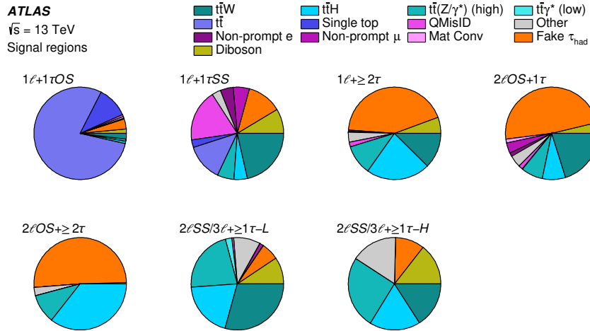
Figure 4. The fractional contributions of the various backgrounds to the total predicted background in each of the seven signal region categories (see section 5). The background estimation methods are described in section 6. The background contributions after the likelihood fit to data under the background-only hypothesis are shown (see section 7).
