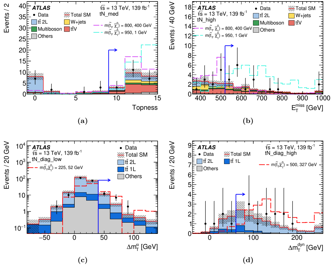
Figure 11. Kinematic distributions in the (a) tN_med, (b) tN_high, (c) tN_diag_low and (d) tN_diag_high SRs. The full event selection in the corresponding signal region is applied, except for the requirement (indicated by an arrow) that is imposed on the variable being plotted. The distributions shown are post-fit, i.e. each background is scaled by a normalisation factor obtained from a background-only likelihood fit to the CRs (see table 14). In addition to the background prediction, a signal model is shown on each plot. The hatched area around the total SM prediction includes statistical and experimental uncertainties. The last (first) bin contains overflows (underflows).
