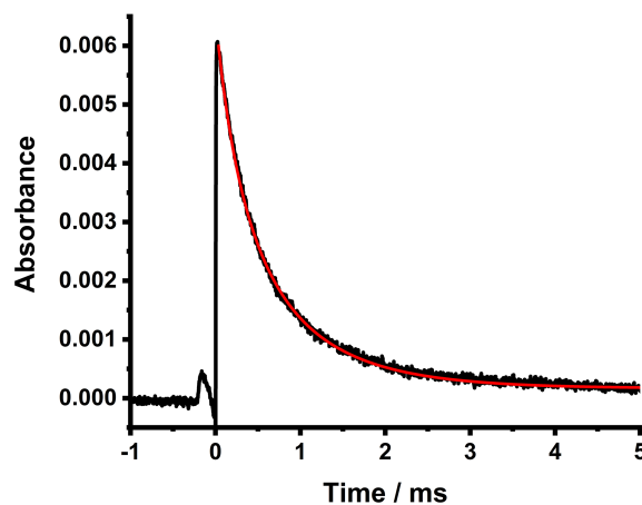
Figure 5. Time-resolved absorbance for \text{CH}_2\text{OO} obtained at a wavenumber of \sim 1285.73 \text{ cm}^{-1} . Data are the average of 1000 photolysis shots at a total pressure of 50 Torr. For these data, [\text{CH}_2\text{I}_2] = 1.6 \times 10^{14} \text{ cm}^{-3} , and [\text{SO}_2] = 0 . The fit to the data using the model containing the reactions given in Table 1 is shown by the solid red line, which gave k_{\text{phys}} = (504 \pm 40) \text{ s}^{-1} and l = (218 \pm 20) \text{ cm} .
