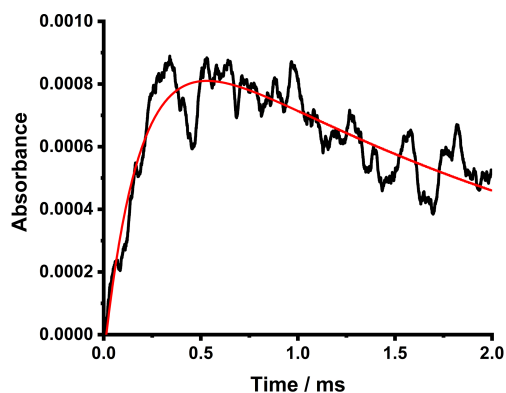
Figure 7. Time-resolved absorbance signals for \text{SO}_3 obtained at a wavenumber of \sim 1388.7\text{ cm}^{-1} . Data are averages of 250 photolysis shots at a total pressure of 50 Torr at 298 K with [\text{SO}_2] = 2.1 \times 10^{14}\text{ cm}^{-3} and [\text{CH}_2\text{I}_2] = 1.6 \times 10^{14}\text{ cm}^{-3} . The fit to Eq. (3) to determine the kinetics describing the production and loss of \text{SO}_3 (red) gave k_{\text{growth}} = (8250 \pm 60)\text{ s}^{-1} and k_{\text{loss}} = (300 \pm 10)\text{ s}^{-1} .
