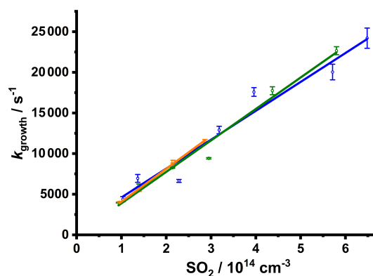
Figure 8. Bimolecular plots of the pseudo-first-order rate coefficients, k_{\text{growth}} , determined from the observed \text{SO}_3 profiles as a function of [\text{SO}_2] . Data were obtained at total pressures of 20 Torr (blue points and line; giving k_5 = (3.55 \pm 0.35) \times 10^{-11}\text{ cm}^3\text{ s}^{-1} , intercept = (1000 \pm 1400\text{ s}^{-1}) ), 50 Torr (green points and line; giving k_5 = (3.87 \pm 0.28) \times 10^{-11}\text{ cm}^3\text{ s}^{-1} , intercept = (100 \pm 900\text{ s}^{-1}) ), and 100 Torr (orange points and line; giving k_5 = (4.05 \pm 0.19) \times 10^{-11}\text{ cm}^3\text{ s}^{-1} , intercept = (400 \pm 400\text{ s}^{-1}) ). The data compare well to the current IUPAC recommendation of (3.70^{+0.45}_{-0.40}) \times 10^{-11}\text{ cm}^3\text{ s}^{-1} (Cox et al., 2020). Error bars are 1\sigma from the fits to Eq. (3).
