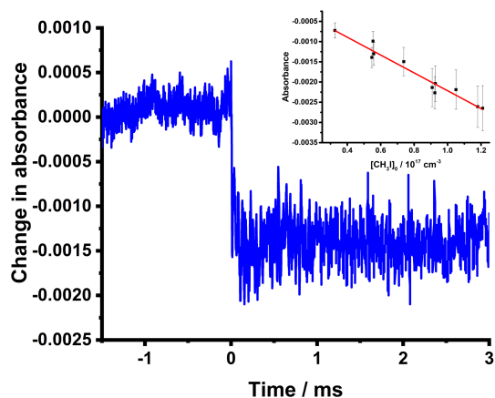
Figure 3. Changes in absorbance at \sim 1287 \text{cm}^{-1} observed on 266 nm photolysis of \text{CH}_3\text{I} . For the data shown in the main figure, [\text{CH}_3\text{I}]_0 = 5.5 \times 10^{16} \text{ cm}^{-3} , p = 50 Torr, and laser fluence is 30 \text{ mJ cm}^{-2} . The data shown are the means of 200 photolysis shots. The inset shows the average post-photolysis ( 0.5 \text{ ms} < t < 3 \text{ ms} ) change in absorbance as a function of the initial \text{CH}_3\text{I} concentration (black points) with the line of best fit (red). The pre-photolysis region for these experiments was defined as -1.5 \text{ ms} < t < -0.5 \text{ ms} .
