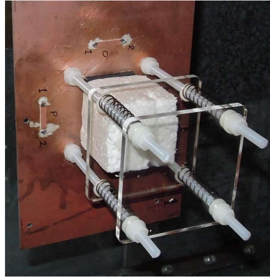
Fig. 3. The spring clamp installed on the SE measurement jig.
