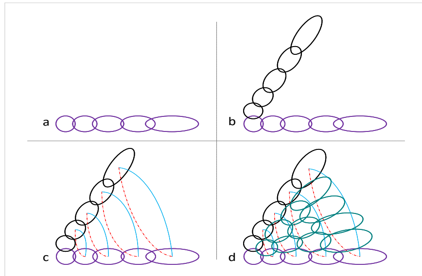
Figure 9. The cell tessellation processes. a) The first step with cells pointing at increasing distance on the x-axis. b) The rotation of the first cells from (a) yielding another set of cells in the second step. c) and d) Show the third and fourth steps where new cells are deployed between the structure in b).
