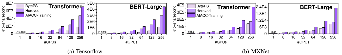
(a) Tensorflow (b) MXNet Fig. 12: Performance on Tensorflow (a) and MXNet (b) for NLP models.
