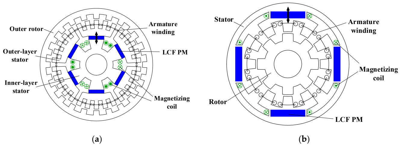
Figure 35. Multi-phase doubly salient VFM machine. (a) Topology decomposition diagrams [92]. (b) Inner rotor topology [96].
