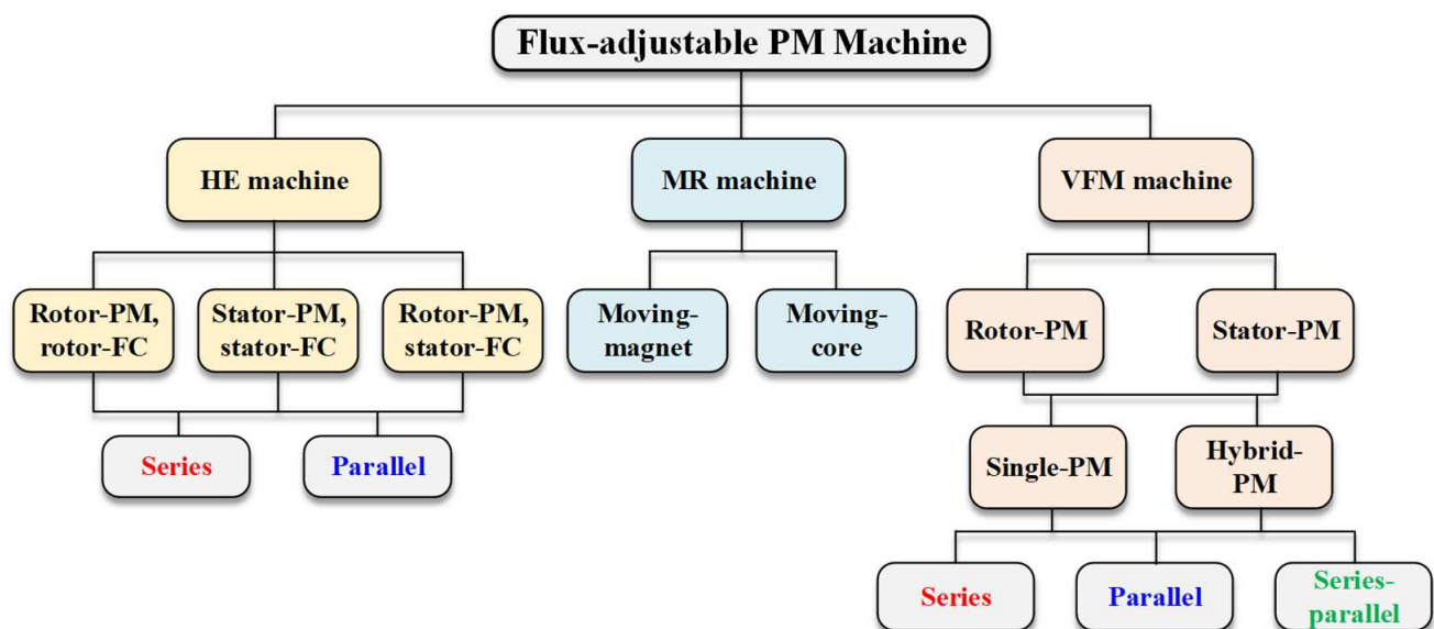
Figure 1. Classification of the flux-adjustable PM machines.
