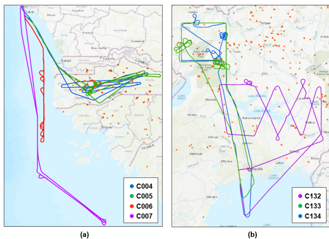
Figure 1. FAAM ARA flight tracks of (a) MOYA-I biomass burning sampling flights C004 (blue), C005 (green), C006 (red), and C007 (purple) over the south-western region of Senegal and the Atlantic seaboard and (b) MOYA-II biomass burning sampling flights C132 (purple), C133 (green), and C134 (blue) over northern Uganda. MODIS infrared satellite retrievals of fires present between (a) 28 February and 2 March 2017 and (b) 28 and 29 January 2019 are also shown (orange triangles). © OpenStreetMap contributors and the GIS user community 2020. Distributed under a Creative Commons BY-SA License.
