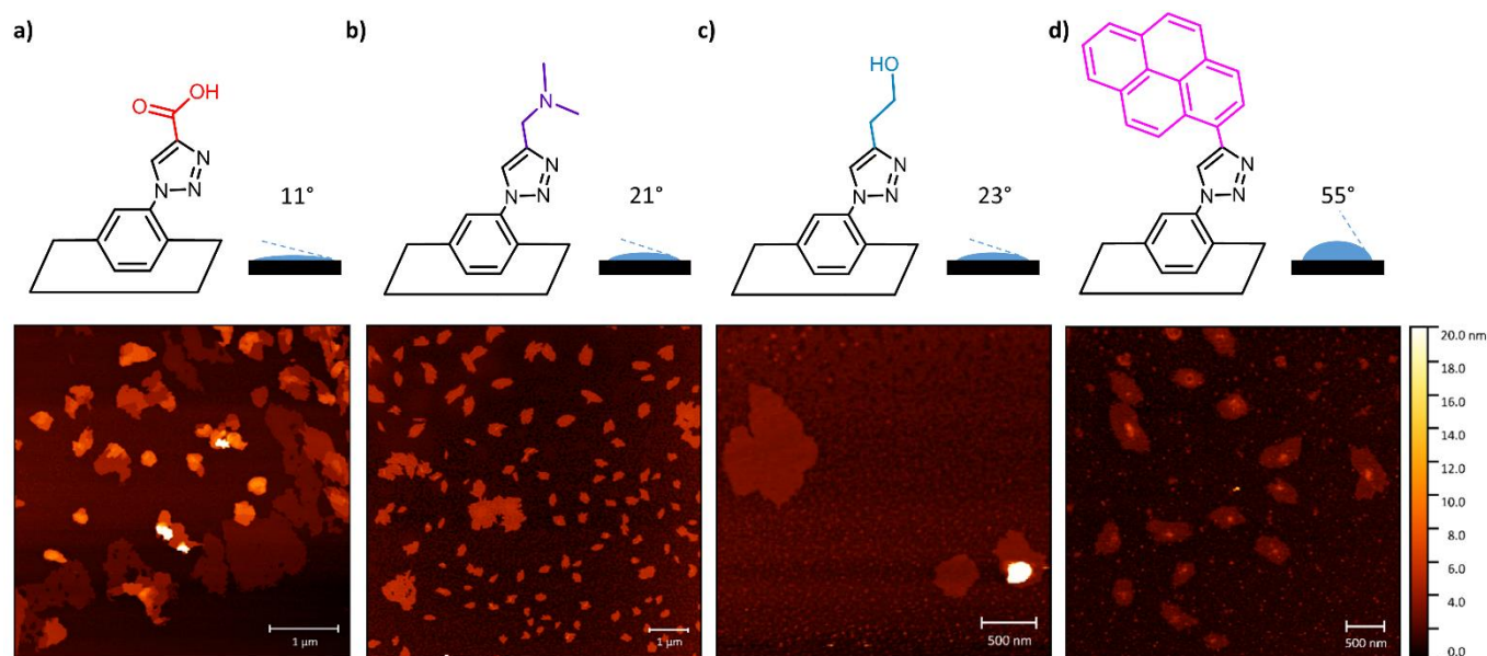
Figure 3. Structural representations, contact angles with water, and AFM topographical images of the obtained a) Cu(BDC-trz-CO 2 H), b) Cu(BDC-trz-NMe 2 ), c) Cu(BDC-trz-OH), and d) Cu(BDC-trz-pyr) nanosheets.
