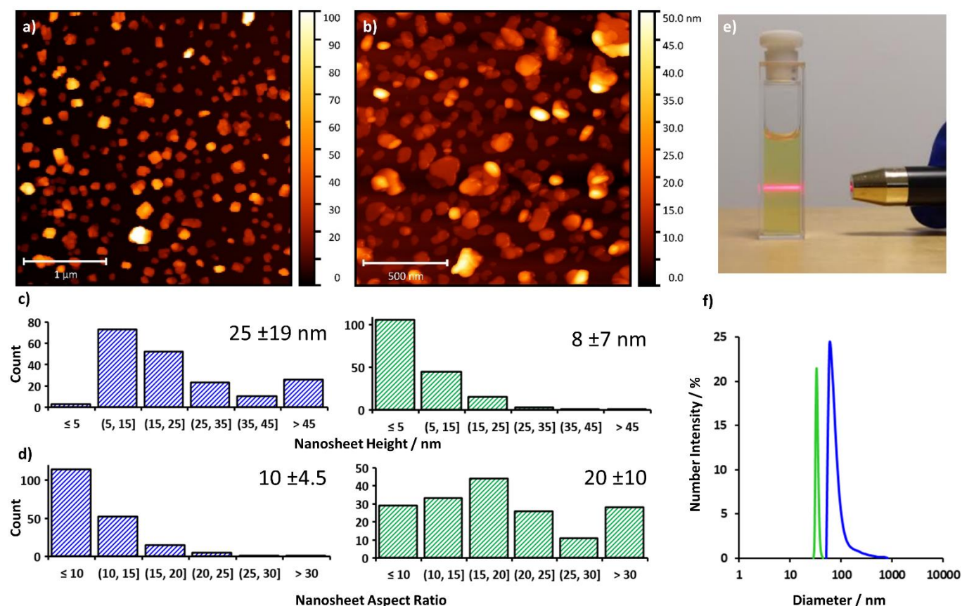
Figure 2. AFM topographical images of a) Cu(NH 2 -BDC) and b) Cu(N 3 -BDC) nanosheets exfoliated in acetonitrile. c) Nanosheet thickness histograms for Cu(NH 2 -BDC) (blue) and Cu(N 3 -BDC)(DMF) nanosheets (green), with inset values for average thickness and standard deviation. d) Nanosheet aspect ratio histograms for Cu(NH 2 -BDC) (blue) and Cu(N 3 -BDC) nanosheets (green), with inset values for average aspect ratio and standard deviation. e) Tyndall scattering images of Cu(N 3 -BDC) nanosheets. f) Particle size distribution data obtained from DLS for Cu(NH 2 -BDC) nanosheets (blue) and Cu(N 3 -BDC) nanosheets (green).
