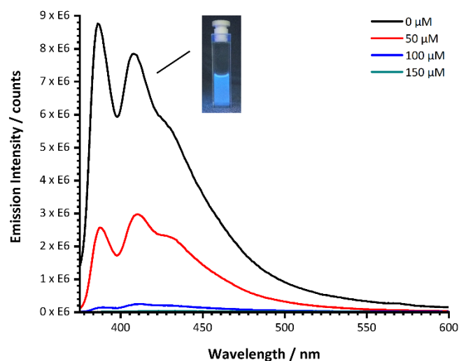
Figure 4. Emission spectra of Cu(BDC-trz-pyr) MONs in acetonitrile with increasing concentrations of nitrobenzene ( \lambda_{\text{ex}} = 351 nm). Inset shows an image of the suspension under a UV lamp.
