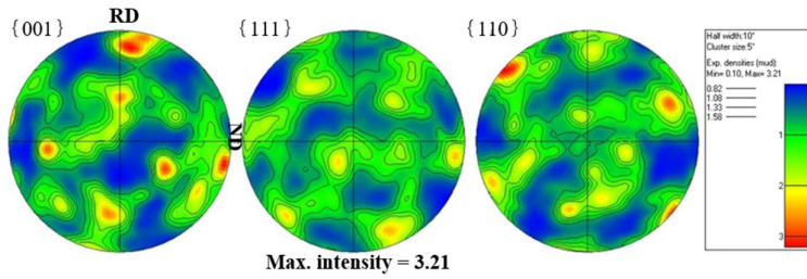
(b) eutectoid rail-transition zone
