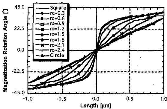
Fig. 4. Numerically calculated domain wall width for rounded squares different radius r_c and also the circular disks and fully square elements.
