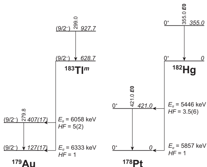
FIG. 8. Partial \alpha -decay schemes for ^{183m}\text{Tl} and ^{182}\text{Hg} . Hindrance factors (HF) for \alpha -decay transitions are given. The data for ^{182}\text{Hg} are taken from [36].
