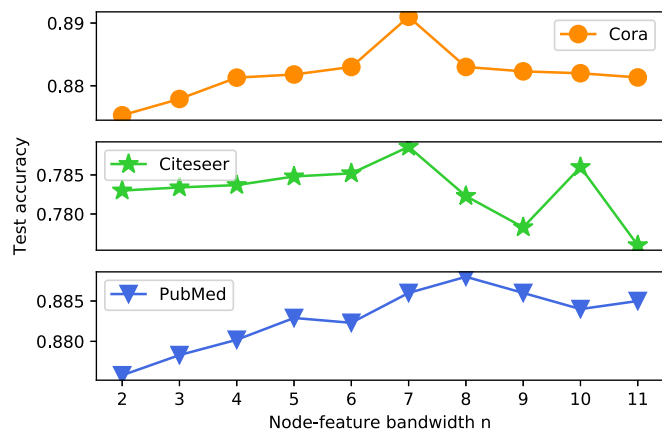
(a) Test accuracy.
