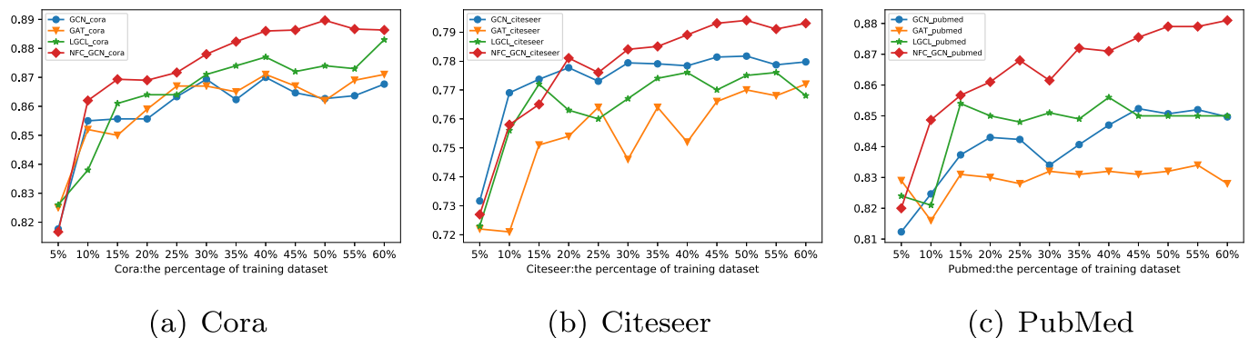
Fig. 10. Effect of training set size. NFC-GCN outperforms others on the whole and it gets more significant improvement with a larger training set.
