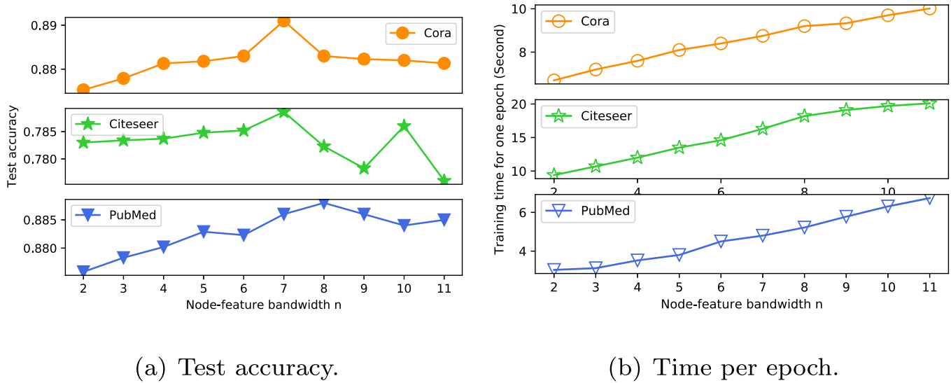
Fig. 8. Effect of node bandwidth n on accuracy and time per epoch.
