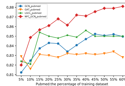
(c) PubMed
