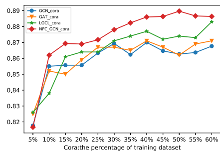
(a) Cora
