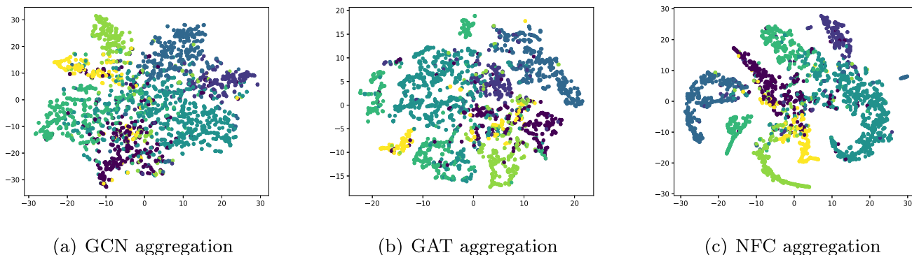
Fig. 7. Visualization of the embeddings on the Cora dataset. We map the embeddings learned from GCN, GAT and NFC aggregation to the 2-D space using t-SNE. Node colors denote classes.
