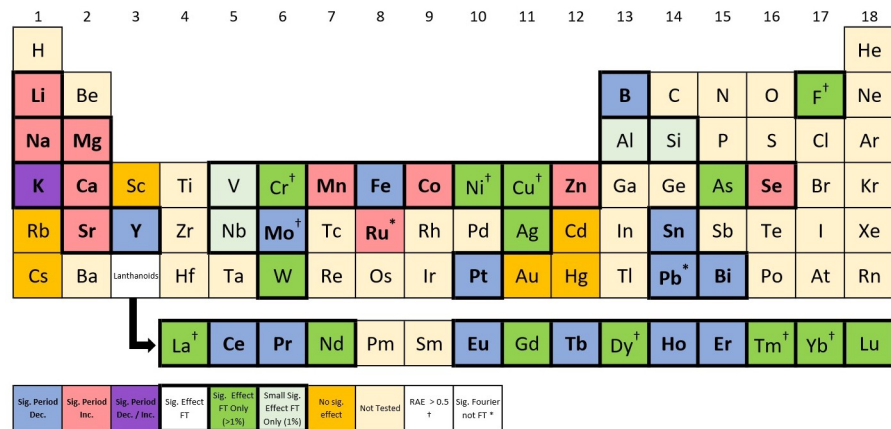
Fig 3. Combined output of FFT–NLLS and LSW–FT methods allows further insight into the impact of excess elements. For each method, an element (see Tables 1–3) is defined as having a significant effect if at least one corresponding chemical treatment gave a significant result (a statistically significant result which also follows the specific method’s usability criteria). Colours/ bold font/ bold outline denote the type of induced change (see key).
