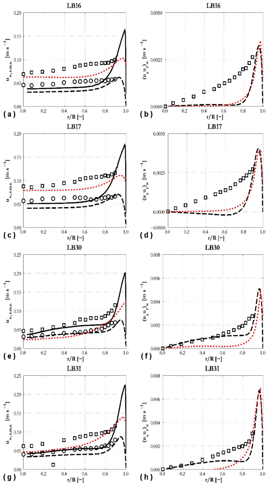
Fig. 6. Predictions of radial profiles of r.m.s. of the water velocity fluctuations (a, c, e, g) and water Reynolds shear stress (b, d, f, h) compared against experiments from Liu and Bankoff (1993a). (a, c, e, g): (□) experiment, u_{w,2r.m.s.} ; (○) experiment, u_{w,r.r.m.s.} ; (-) UoL, u_{w,2r.m.s.} ; (--) UoL, u_{w,r.r.m.s.} ; (●●) HZDR. (b, d, f, h): (□) experiment; (-) UoL; (●●) HZDR.
