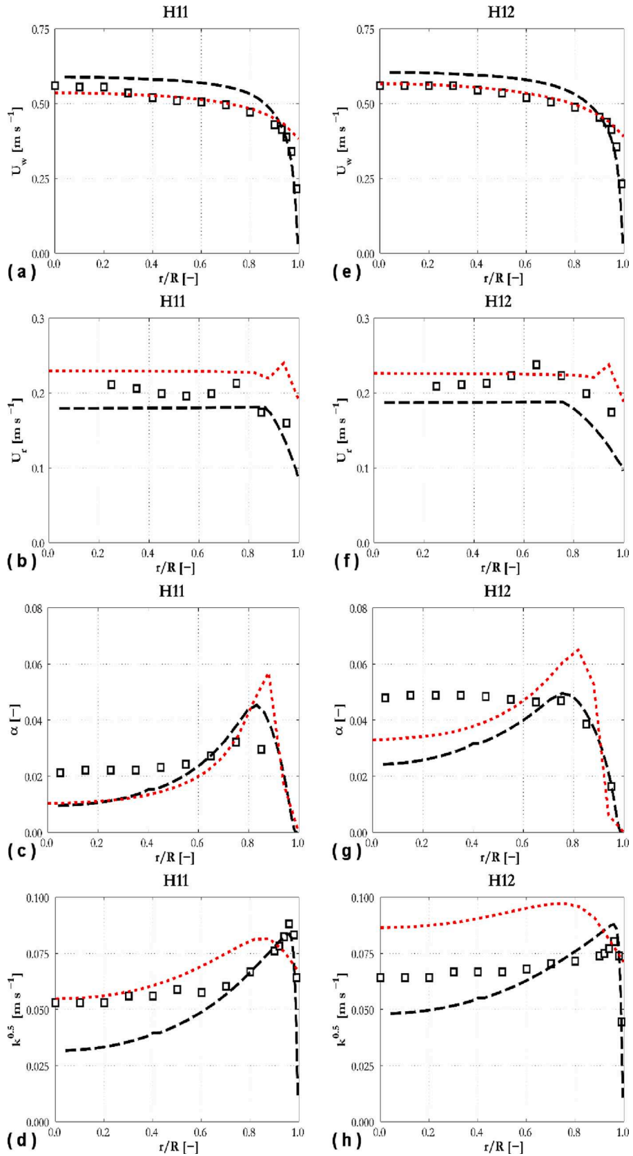
Fig. 1. Predictions of radial profiles of water velocity (a, e), relative velocity (b, f), void fraction (c, g) and turbulence kinetic energy (d, h) compared against experiments H11 and H12 from Hosokawa and Tomiyama (2009): (□) experiment; (---) UoL; (●●●) HZDR.
