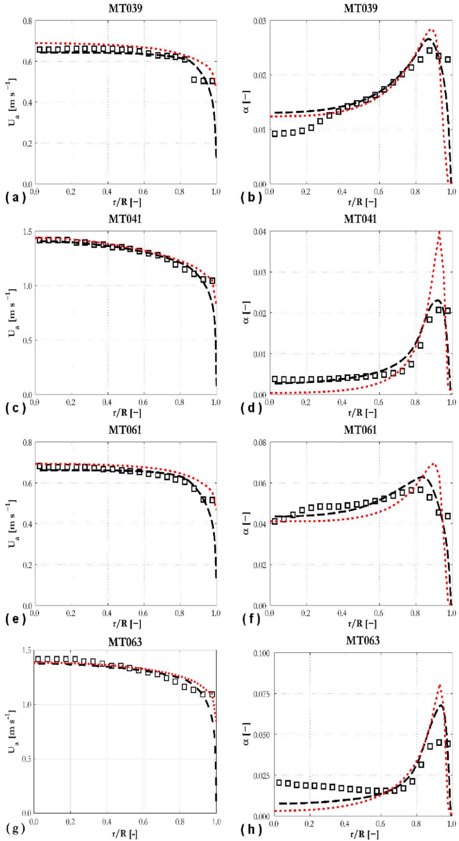
Fig. 4. Predictions of radial profiles of air velocity (a, c, e, g) and void fraction (b, d, f, h) compared against experiments from MTLoop (Lucas et al., 2005): (□) experiment; (---) UoL; (●●●) HZDR.
