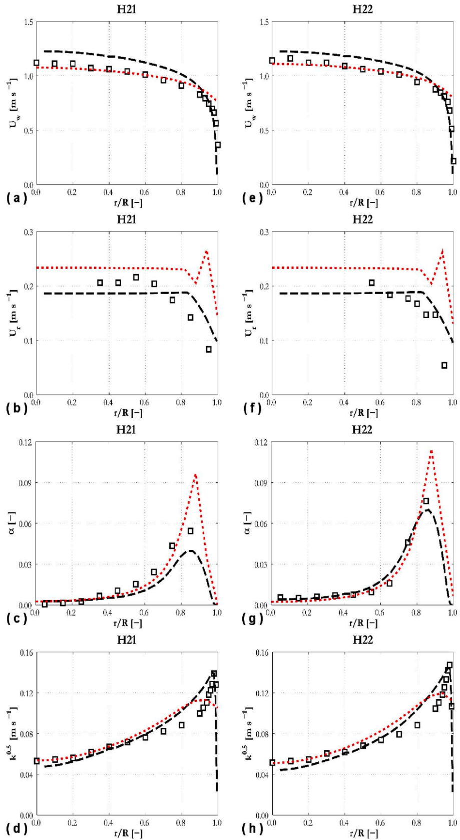
Fig. 2. Predictions of radial profiles of water velocity (a, e), relative velocity (b, f), void fraction (c, g) and turbulence kinetic energy (d, h) compared against experiments H21 and H22 from Hosokawa and Tomiyama (2009): (□) experiment; (---) UoL; (●●●) HZDR.
