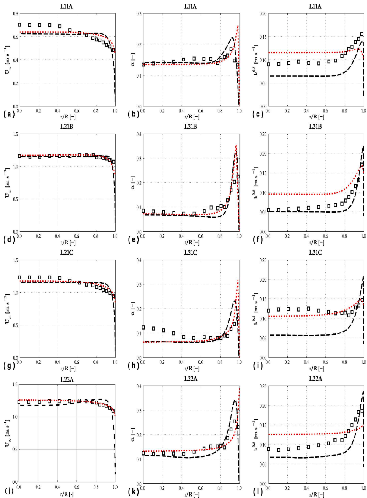
Fig. 3. Predictions of radial profiles of water velocity (a, d, g, j), void fraction (b, e, h, k), and turbulence kinetic energy (c, f, i, l) compared against experiments from Liu (1998): ( \square ) experiment; (---) UoL; (•••) HZDR.
