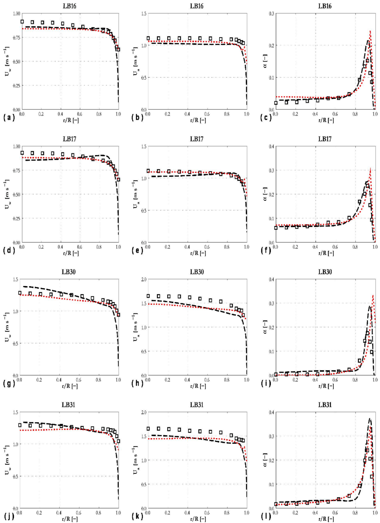
Fig. 5. Predictions of radial profiles of water velocity (a, d, g, j), air velocity (b, e, h, k) and void fraction (c, f, i, l) compared against experiments from Liu and Bankoff (1993a): (□) experiment; (---) UoL; (●●●) HZDR.
