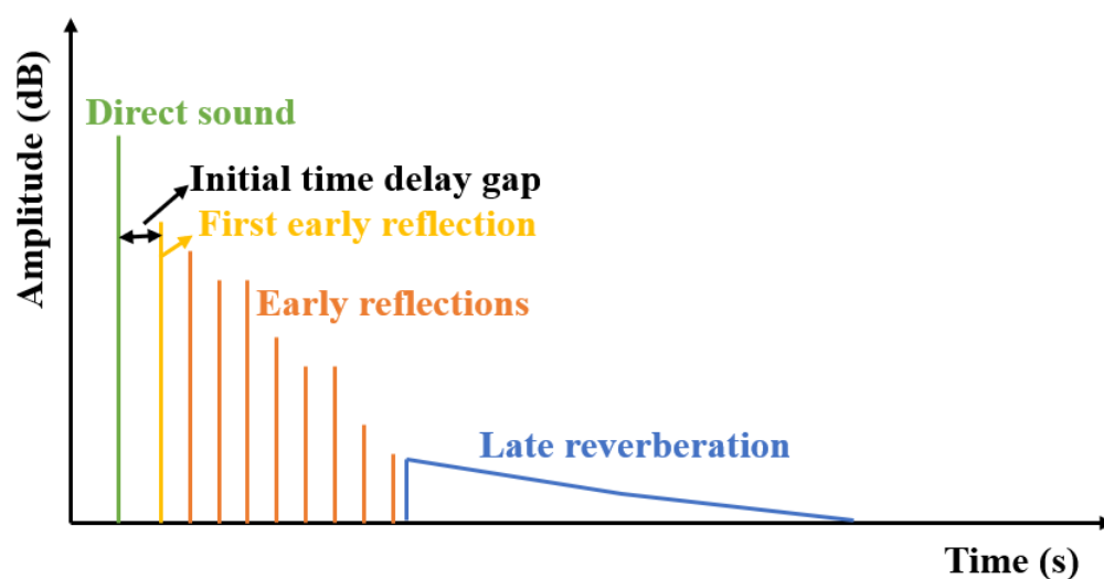
Figure 1. Representation of a room impulse response.
