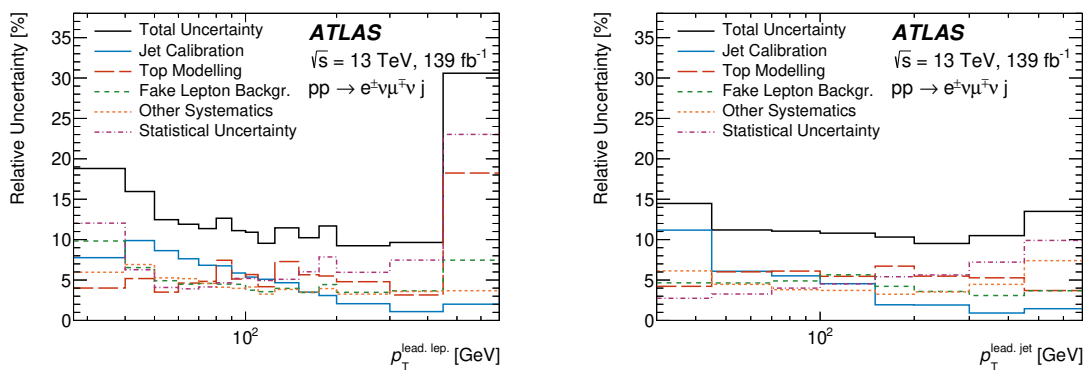
Figure 4. Relative size of uncertainties for the unfolded p_T^{\text{lead. lep.}} and p_T^{\text{lead. jet}} distributions. “Jet Calibration” uncertainties encompass jet energy scale and resolution uncertainties while “Top Modelling” encompasses all t\bar{t} and single-top modelling uncertainties. “Fake Lepton Backgr.” is the uncertainty in the non-prompt-lepton estimate from the fake-factor method. “Other Systematics” includes modelling and total cross-section uncertainties in the remaining backgrounds, lepton-related uncertainties as well as uncertainties due to pile-up reweighting and the signal modelling in the unfolding, while “Statistical Uncertainty” is the combined statistical uncertainty in the signal region, from control regions, and from MC simulations.
