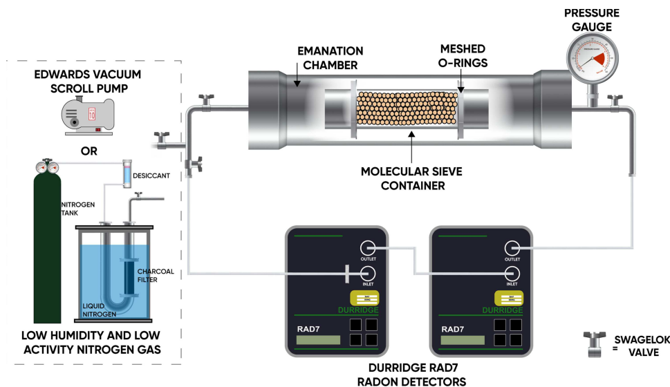
Figure 3. Schematic of the setup used for the radon emanation tests.
