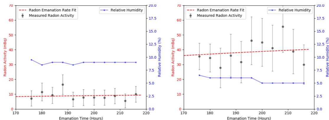
Figure 4. Plot of radon concentration as a function of emanation time. NU-developed MS on the left and Sigma-Aldrich MS on the right.
