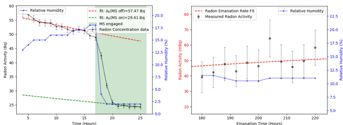
Figure 8. Plot of the change in radon concentration observed while using the powdered NU-developed MS (left) and a plot of radon concentration as a function of emanation time (right) in the powdered NU-developed MS emanation test.
