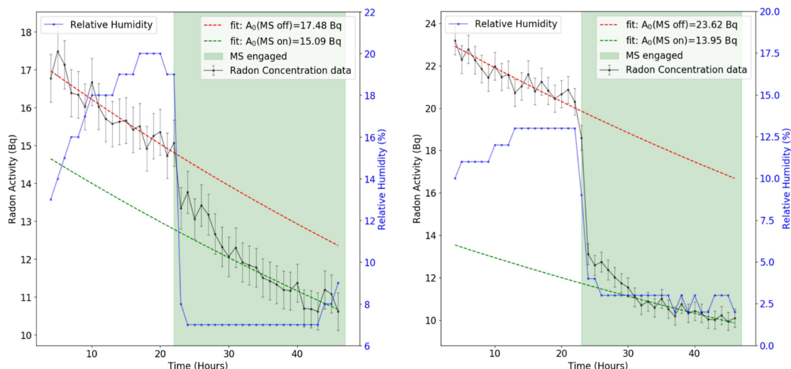
Figure 6. Plot of the change in radon concentration observed due to application of molecular sieve. NU-developed MS on the left and Sigma-Aldrich MS on the right.
