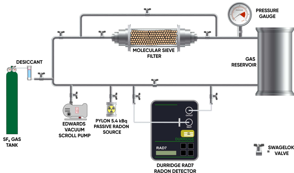
Figure 5. Schematic of the setup used for the radon filtration tests.
