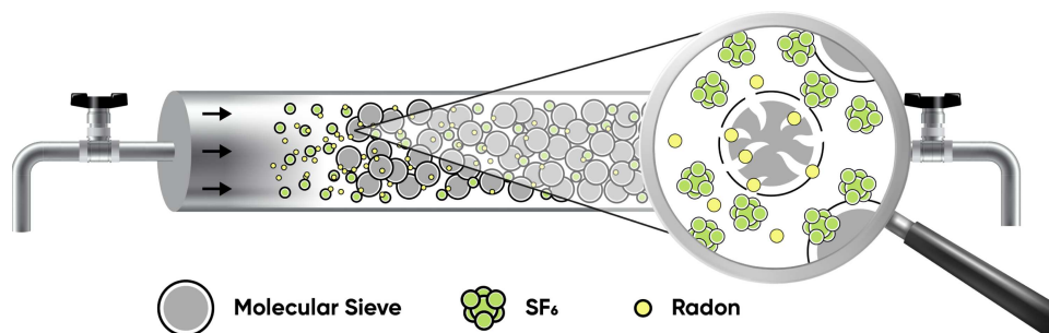
Figure 1. Illustration of the separation of smaller radon atom from larger \text{SF}_6 molecules using MS. The arrows represent the direction of flow of the gas inside the molecular sieve vessel.
