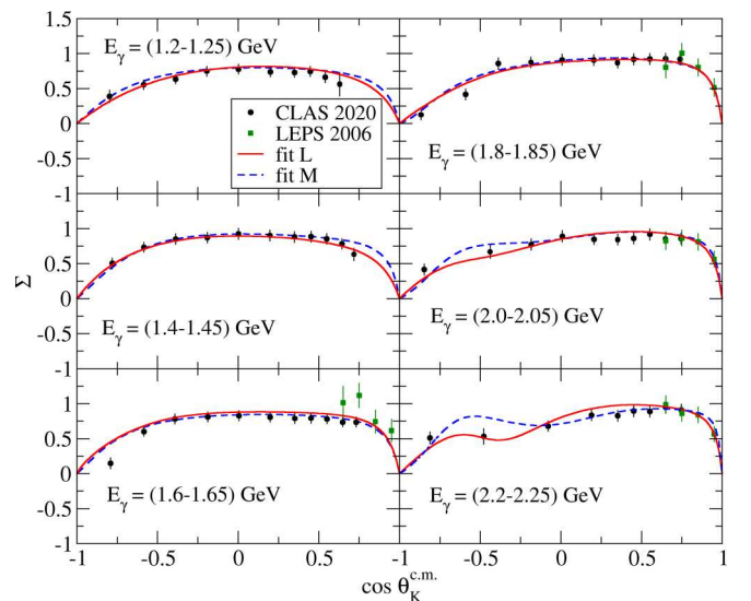
FIG. 6. The photon beam asymmetry for several energetic bins in dependence on the kaon center-of-mass angle \theta_K^{c.m.} as calculated by the best fit achieved by the MINUIT alone and by the LASSO method and compared with the CLAS [12] data. Notation of the curves is the same as in Fig. 2.
