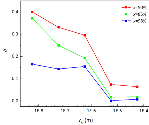
Fig. 11. The relative error of droplet wetting rate simulated by the standard VOF method and present multiscale method.
