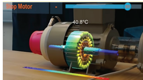
(b) Digital twin
