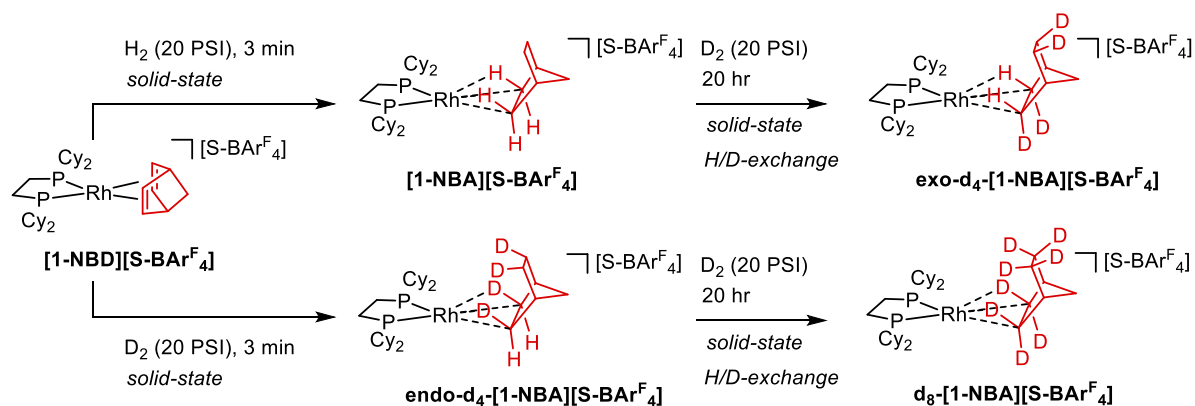
Figure S7. Syntheses of \text{d}_x\text{-[1-NBA][S-BAr}^F_4] ( x=0, 4, 8 ).
