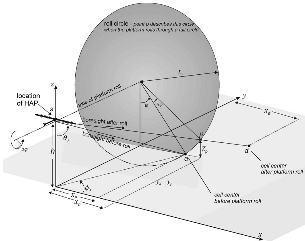
Fig. 2. Change in antenna pointing angles following platform roll \Delta\varphi .
