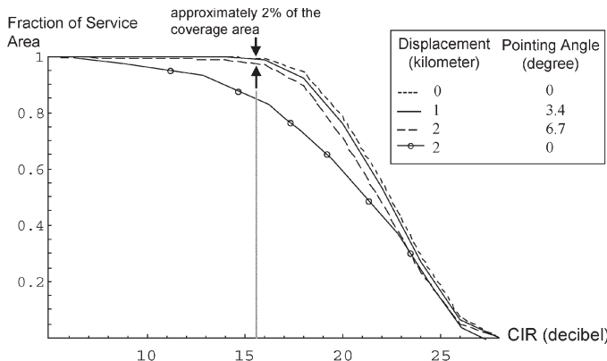
Fig. 6. Effect of platform drift: fractional coverage on any of the four channels for the entire service area for different choices of antenna pointing correction.
