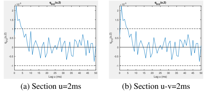
Fig. 1. (a) and (b) are section of this peak along the vertical and horizontal direction, along with the confidence limit (two dashed horizontal lines) and null value (solid horizontal line) based on the assumption of uncorrelated spike trains.
