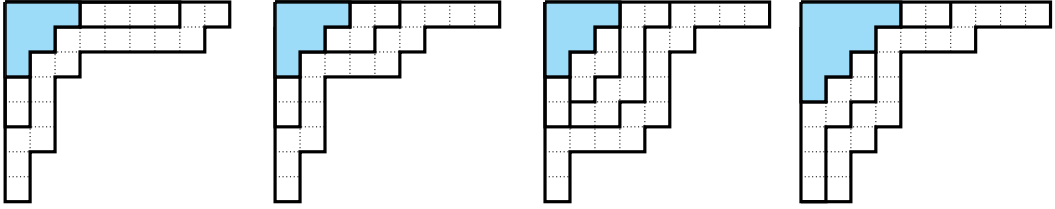
FIGURE 2. Examples of partitions which label height 0 characters for \mathfrak{S}_{28} and \mathfrak{S}_{36} (and therefore label constituents of Saxl’s tensor square by Theorem B). There are 672 and 1417 such characters for these groups, respectively. A combinatorial construction of all such partitions (for arbitrary n \in \mathbb{N} ) is given in Subsection 1.4.
