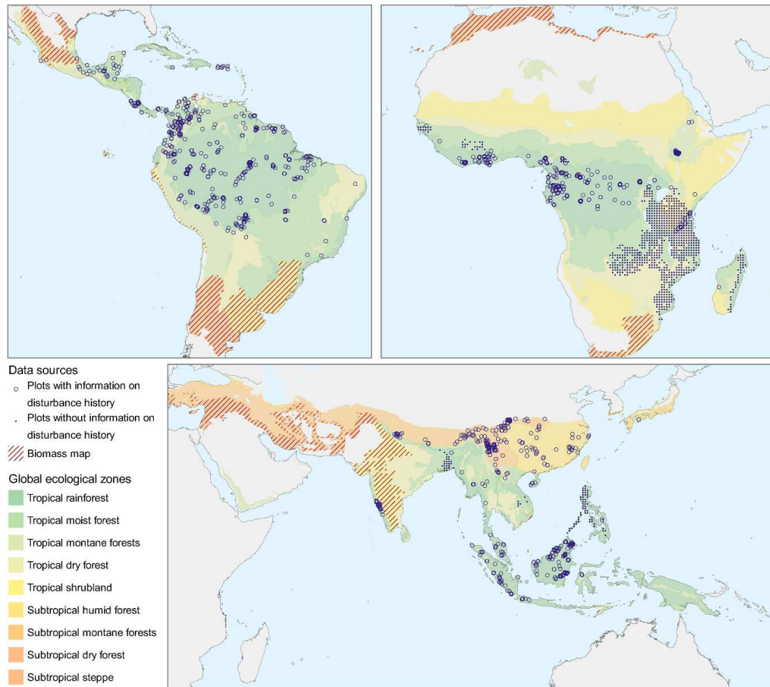
Figure 2. Overview of locations of plots with information on disturbance history and plots without information on disturbance history (mostly data from NFIs), as well as the FAO global ecological zones (FAO 2012) for which the refined default biomass values were estimated based on a global biomass map.
