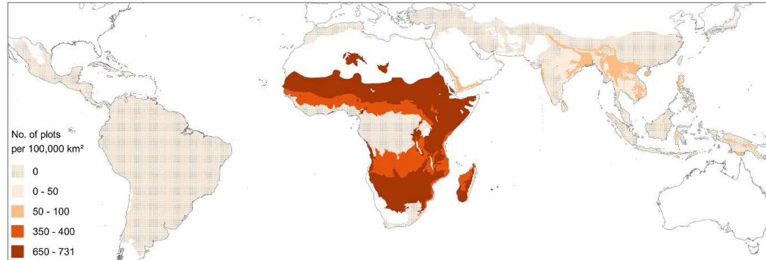
Figure 5. Number of plots per 100 000 km 2 of natural forests per ecological zone. Natural forest areas per ecological zone were based on Schulze et al (2019). We recommend targeted data collection in areas with low sampling intensity, particularly to increase the number of plots with information on disturbance history. (a) Plots with information on disturbance history; (b) plots without information on disturbance history.
