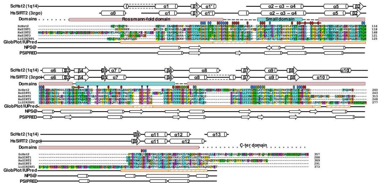
Fig 2. Multiple sequence alignments of LiSIR2RP1 with yeast Hst2 and human SIRT1-3 homologues. Multiple sequence alignment of LiSIR2rp1 (Uniprot #Q816E4) with ScHst2 (P53686), hSIRT1 (Q96EB6), hSIRT2 (Q81XJ6) and hSIRT3 (Q9NTG7) (ScHst2 region 1–228 and 517–747 and hSIRT3 1–108 were omitted for clarity). Above the alignment, boxes define the Rossmann-fold (pink), and the small domain (blue). The main secondary structure elements described in ScHst2 (pdb: 1q14) and hSIRT2 (pdb: 3zgo) are indicated. Important residues are pointed: residues important for binding of the NAD (blue circle), acetyl-lysine peptide (green circle) and Zinc ion (blue triangle) and identified as hot-spot by Parenti et al. (red circle) [56]. ECS site and selectivity binding pocket are delimited by a red line. Results of globular domain predictions by GlobPlot and IUPred are depicted as orange boxes (full colored in case of consensus between both algorithm and hachured when identified by only one). Results of secondary structure predictions by NPS@ and PSIPRED are represented beneath ( \beta sheets are indicated with arrows and \alpha helices with cylinders).
