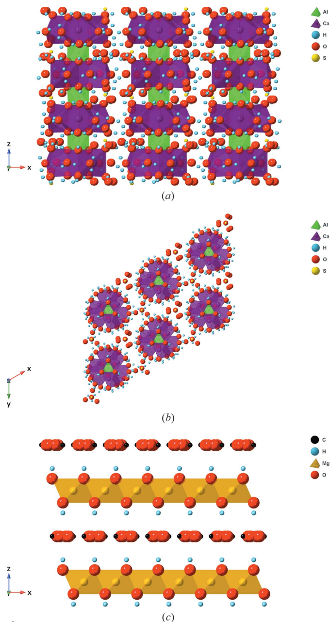
Figure 1 Representation of the ettringite crystal structure shown down the y ( b ) axis [panel (a)] and the z ( c ) axis [panel (b)] (Goetz-Neunhoeffler & Neubauer, 2006). Panel (c) shows a 'cross-sectional' view of the hydrotalcite LDH structure shown down the y ( b ) axis (Radha et al. , 2007), where Mg = Mg or Al. Not to scale.
