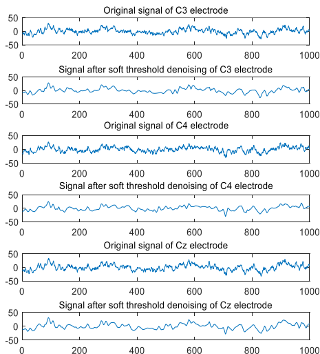
Fig. 5. De-noising results of WT method (typical electrodes).
