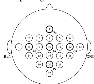
Fig. 2. Schematic diagram of EEG electrode position.
