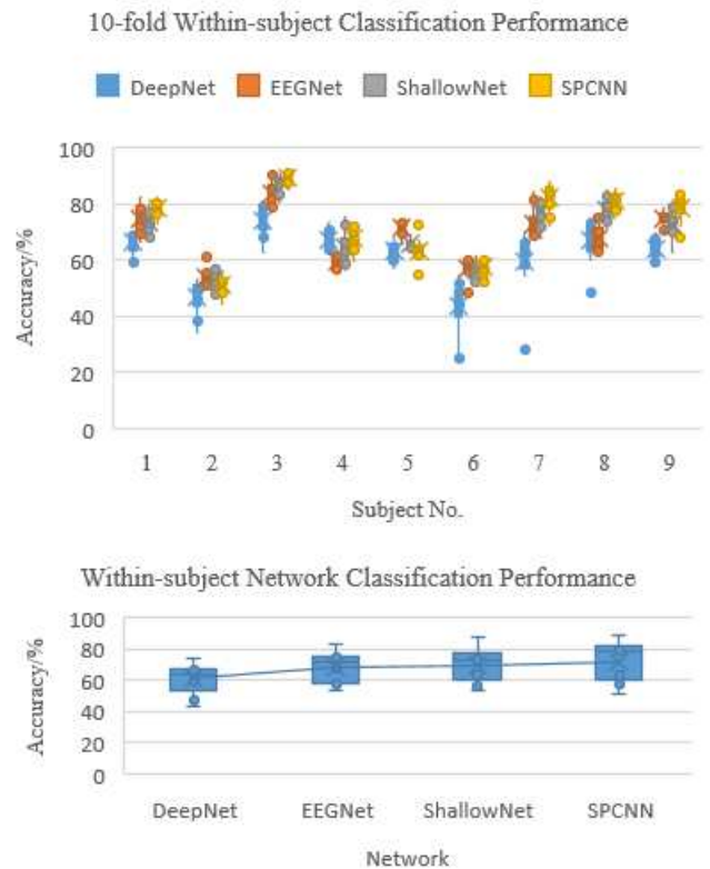
Fig. 6. Within-subject testing classification performance. (a) 10-fold cross classification performance; (b) Network classification performance.
