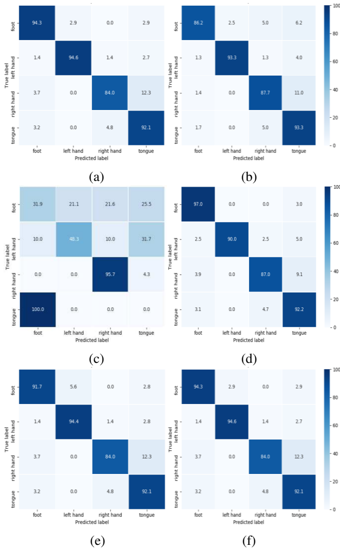
Fig. 7. Confusion matrixes of the SPSCNN evaluated with different frequency bands filtered. (a) Unfiltered (Acc=90.97%); (b) \alpha band filtered (Acc=89.93%); (c) \beta band filtered (Acc=40.28%); (d) \gamma_1 band filtered (Acc=91.32%); (e) \gamma_2 band filtered (Acc=90.28%); (f) \gamma_3 band filtered (Acc=90.97%).
