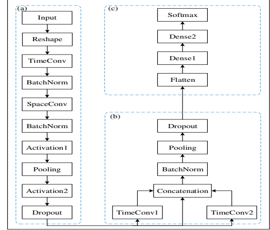
Fig. 4. Hierarchical framework of SPCNN. (a) Serial feature extraction module: input deformation, extraction of time domain, spatial domain and frequency domain characteristics; (b) Parallel feature extraction module: depth characteristics extraction at different scales; (c) Classification module: category determination of signal.
