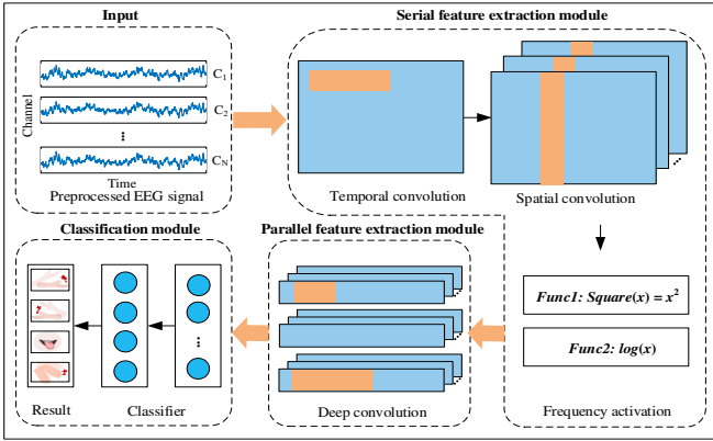
Fig. 3. Main structure of SPCNN.
