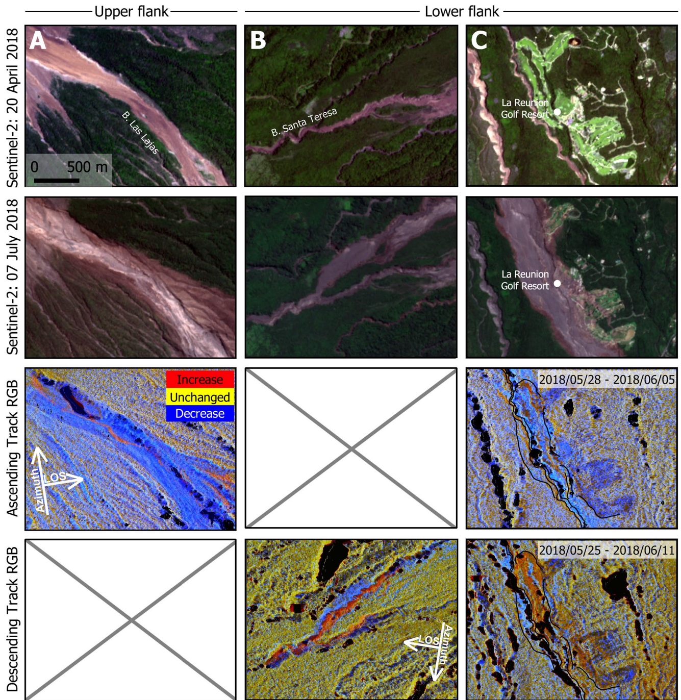
Figure 4. Backscatter changes associated with the June 3, 2018 eruption in different sections of the drainage systems. Pre- and post-eruption optical imagery and ascending CSK RGB image of (a) eastern summit area affected by PDCs in Barranca Las Lajas and (b) the lower section of Barranca Santa Teresa showing the June 3 PDCs infill and overtop (overbank) the drainage system. Blue and red overlays indicate the increases and decreases in backscatter observed from the RGB images. (c) Pre- and post-eruptive optical imagery, descending and ascending CSK RGB images over the La Réunion golf course and Barranca Las Lajas showing backscatter changes correlated with different satellite look direction and incidence angle. Areas not covered by corresponding SAR image are indicated by a gray cross. Location of the scene is shown in Figure 1c.
