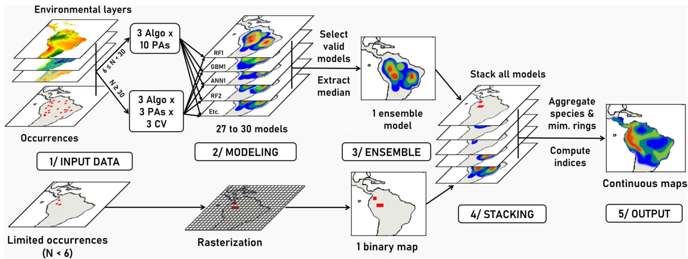
FIGURE 2 Species Distribution Model (SDM) workflow depicting the different analytical steps performed. Distribution models are computed for each OMU. Depending on sample size, modelling steps and settings differed. Clipping step to constrain SDM projections to plausible distribution ranges is not shown on the chart. Algo = algorithms used in the study, namely random forest (RF), gradient boosting models (GBM) and artificial neural networks (ANN); PAs = sets of pseudo-absences; CV = cross-validation folds; mim. rings = mimicry rings
