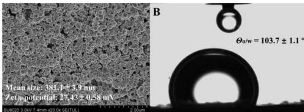
Figure 1. Morphology (A) and interfacial wettability (B) of ZCPs.
