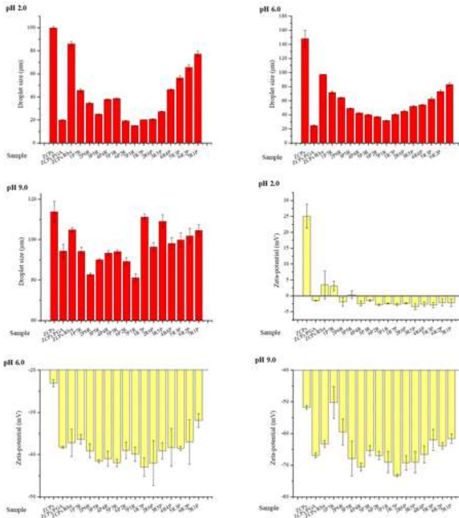
Figure 4. Influence of different pH values on the droplet size and zeta-potential of Pickering emulsions co-stabilized by ZCPs, PGA, and Rha.
