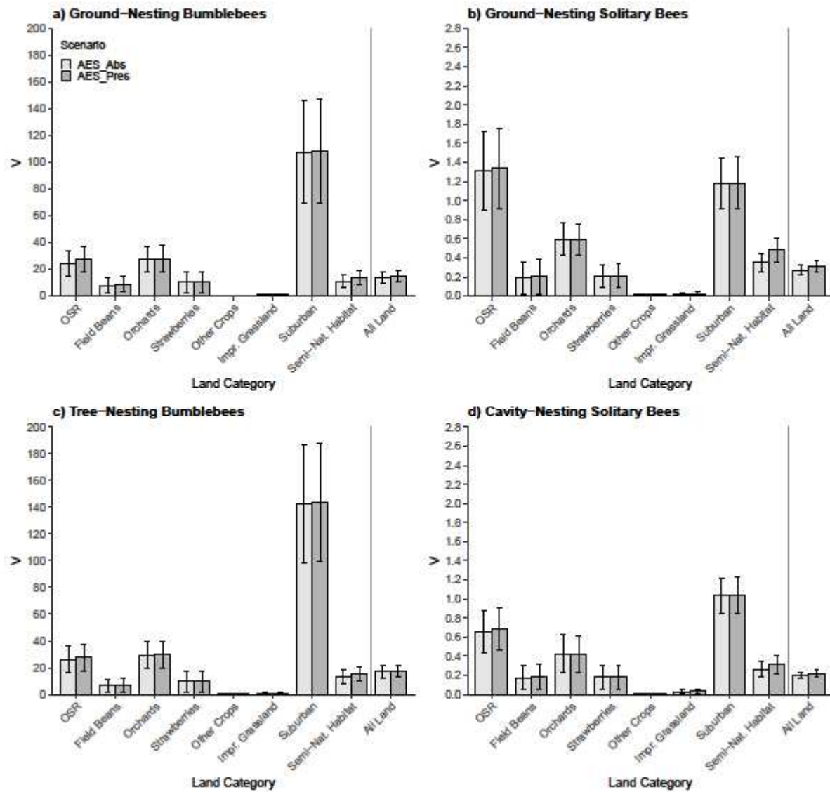
Figure S9: Late Spring visitation (V) by land category, scenario, and guild. V represents the number of visits received on average per cell (25m 2 ) of that land category in England during this season. Late spring: late April/early May - early/mid-June.
