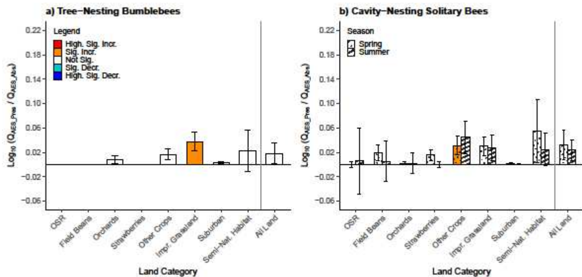
Figure S1: Predicted impact of Agri-environment schemes (AES) on nest productivity ( Q ; production of new reproductive females per 25\text{m}^2 ) nationally to all land categories and subdivided by land category for (a) tree-nesting bumblebees and (b) cavity-nesting solitary bees (separated by active season). The impact is measured as the log of the ratio between the scenarios with AES features present and absent. Significance thresholds are number of standard deviations that the log ratio is above (increase) or below (decrease) zero: value \geq |3| is highly significant, |2| \leq \text{value} < |3| is significant.
