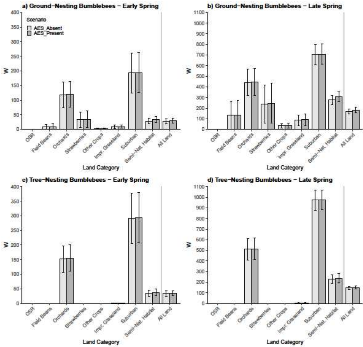
Figure S7: Worker generation ( W ) by land category, scenario, and bumblebee guild. W represents the number of new workers produced on average per cell ( 25m^2 ) of that land category in England during the captioned season and thus foraging in the next season.
