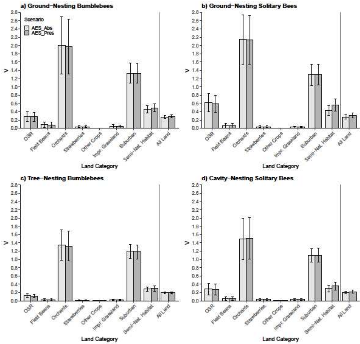
Figure S8: Early Spring visitation (V) by land category, scenario, and guild. V represents the number of visits received on average per cell (25m 2 ) of that land category in England during this season. Early spring: early/mid-March – late April/early May.
