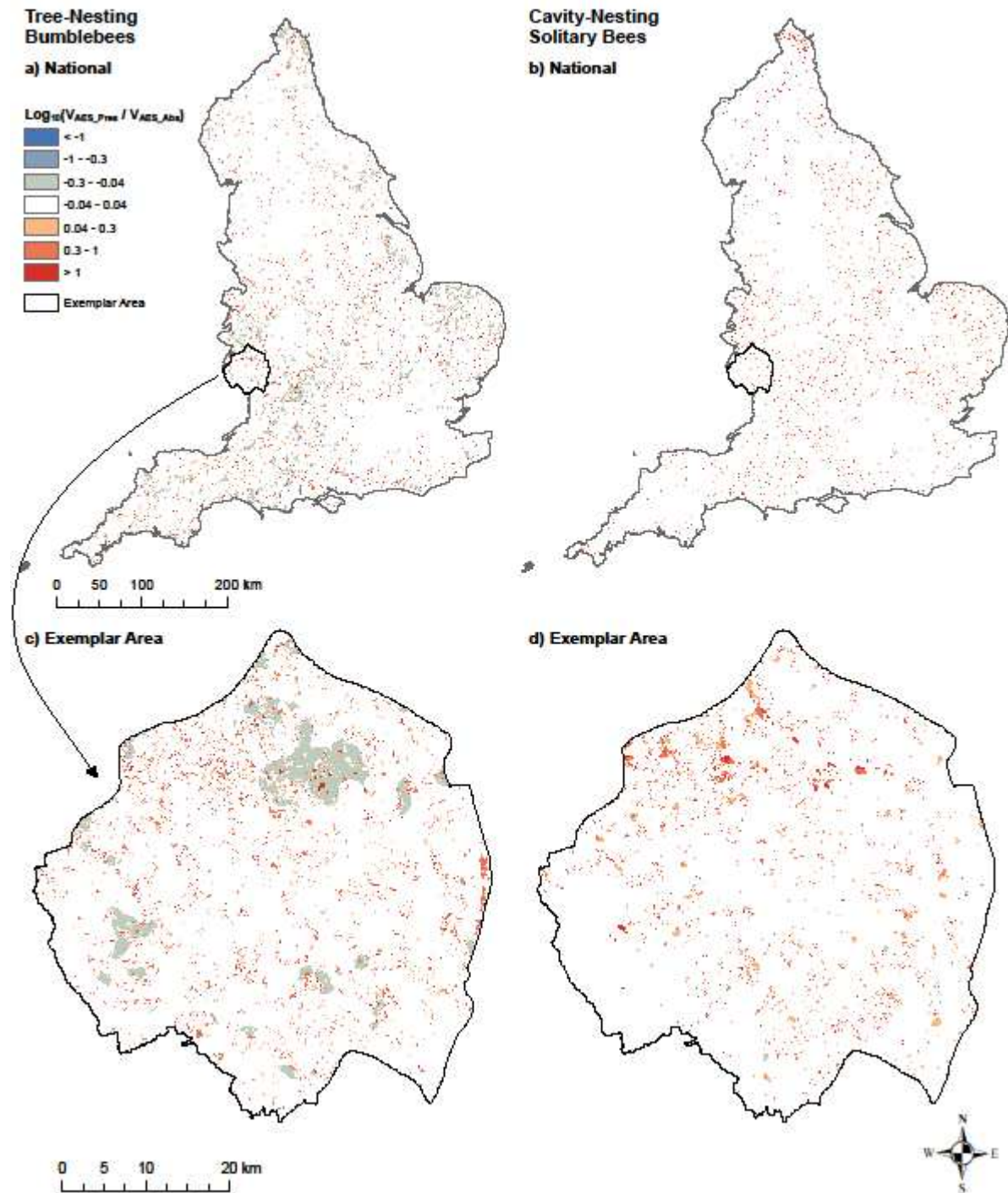
Figure S17: Impact of Agri-environment schemes on floral visitation rate (V) for tree and cavity-nesting guilds in England for early spring 2016 at national scale (a, b) and for an exemplar area (c, d) in western England. The impact is shown as the log of the ratio of V (visitation/25m 2 ) between scenarios with AES present and absent. Only cells with significant change are shown - where the log ratio is at least 2 standard deviations from zero. Early spring: early/mid-March – late April/early May.
