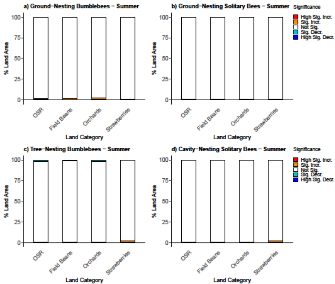
Figure S12: Percentage of land area in significance thresholds for predicted impact of Agri-environment schemes (AES) on floral visitation rate ( V ; visits per 25m^2 cell) nationally to all guilds in summer. The impact is measured as the log ratio between the scenarios with AES feature present and absent. Significance thresholds are number of standard deviations that the log ratio is above (increase) or below (decrease) zero: value \geq |3| is highly significant, |2| \leq \text{value} < |3| is significant. Summer: early/mid-June - early/mid-September
