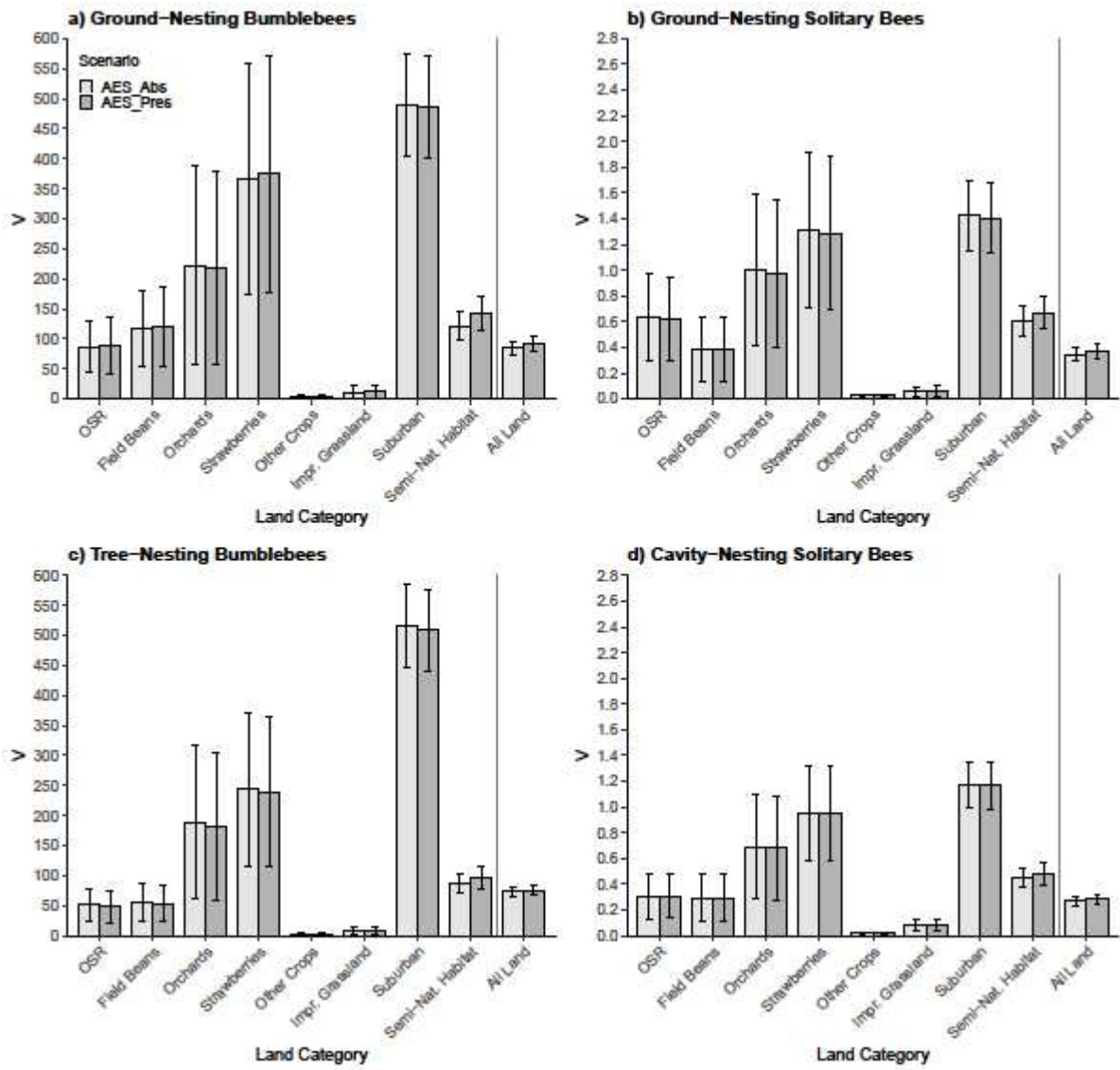
Figure S10 : Summer visitation ( V ) by land category, scenario, and guild. V represents the number of visits received on average per cell ( 25m^2 ) of that land category in England during this season. Summer: early/mid-June – early/mid-September.
