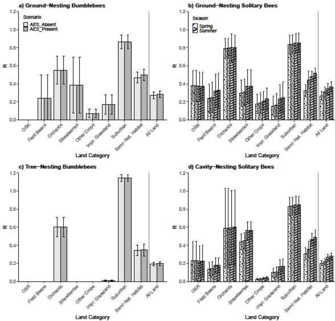
Figure S6: Nest density ( R ) by land category, scenario, and guild. R represents the number of nests found on average per cell ( 25m^2 ) of that land category in England at the beginning of the active season for the next year.
