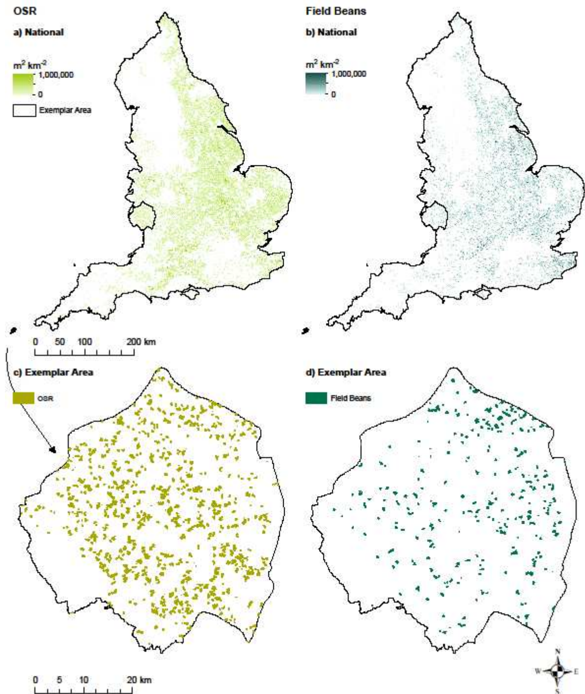
Figure S13: Geographical distribution of OSR and field beans across England (a, b) and an exemplar area (c, d) in 2016. The national maps show crop density (m 2 ) within a 1km 2 grid. The exemplar area maps show actual features.
