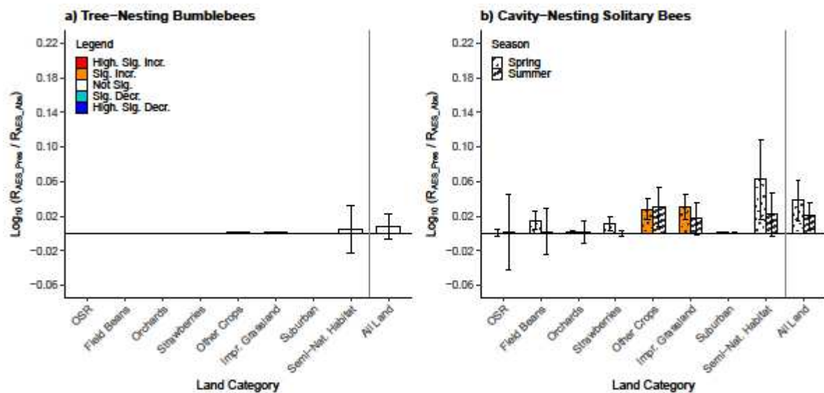
Figure S2: Predicted impact of Agri-environment schemes (AES) on nest density ( R ; nests per 25\text{m}^2 cell) nationally to all land categories and subdivided by land category for (a) tree-nesting bumblebees and (b) cavity-nesting solitary bees (separated by active season). The impact is measured as the log of the ratio between the scenarios with AES features present and absent. Significance thresholds are number of standard deviations that the log ratio is above (increase) or below (decrease) zero: value \geq |3| is highly significant, |2| \leq \text{value} < |3| is significant.
