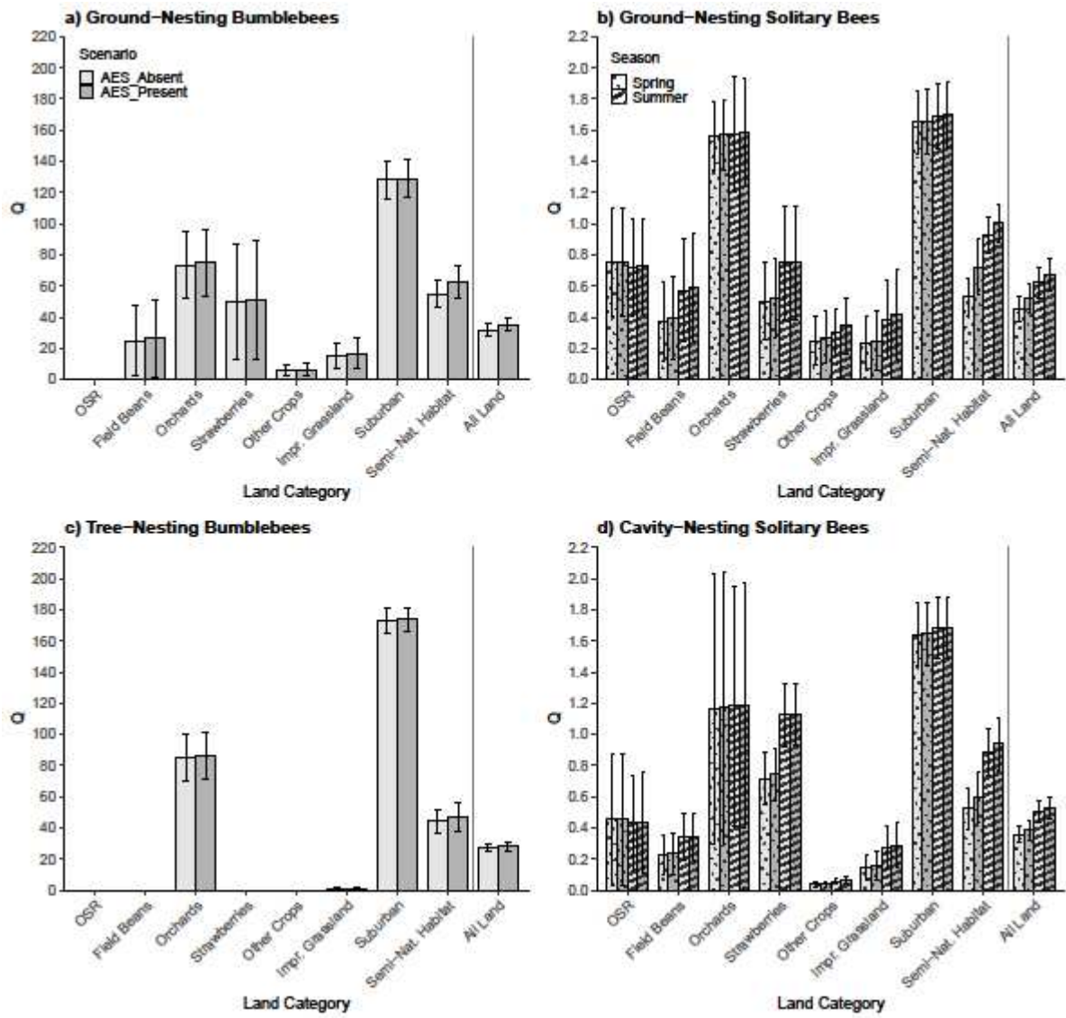
Figure S5: Nest productivity ( Q ) by land category, scenario, and guild. Q represents the number of new reproductive females produced on average per cell ( 25m^2 ) of that land category in England at the end of the active season for that year.
