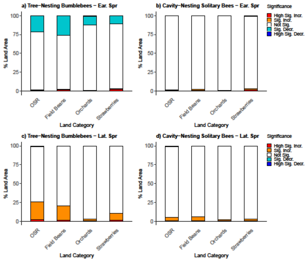
Figure S11: Percentage of land area in significance thresholds for predicted impact of Agri-environment schemes (AES) on floral visitation rate ( V ; visits per 25\text{m}^2 cell) nationally to selected land categories for tree and cavity-nesting guilds in early (a,b) and late (c,d) spring. The impact is measured as the log ratio between the scenarios with AES feature present and absent. Significance thresholds are number of standard deviations that the log ratio is above (increase) or below (decrease) zero: value \geq |3| is highly significant, |2| \leq \text{value} < |3| is significant. Early spring: early/mid-March - late April/early May; Late spring: late April/early May - early/mid-June.
