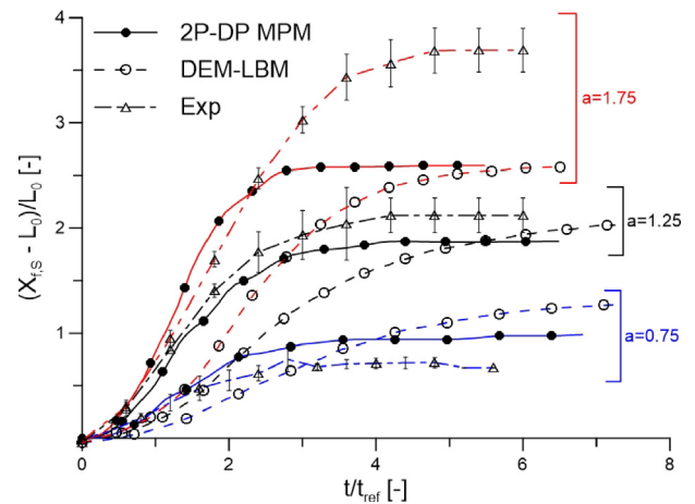
Fig. 10. Evolution of normalized front position in time for different aspect ratios. Numerical results (hollow circles for DEM-LBM and full circles for 2P-DP MPM) and experimental results (triangles) in saturated conditions.
