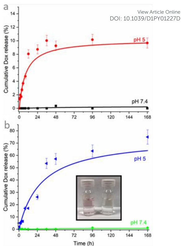
Fig. 4. (a) Cumulative amount of Dox released over time from CND/CaNP-ABPA-PPhe 4 - b -PSar 16 in PBS buffer solution at pH 7.4 (■) and acetate buffer solution at pH 5 (●). (b) Cumulative amount of Dox released over time from CND/CaNP-HUPA-PSar 23 in PBS buffer solution at pH 7.4 (◆) and acetate buffer solution at pH 5 (▲). Inset: buffer solutions outside the dialysis tubing of CND/CaNP-HUPA-PSar 23 at pH 5 (left) and 7.4 (right) after 168 h.
