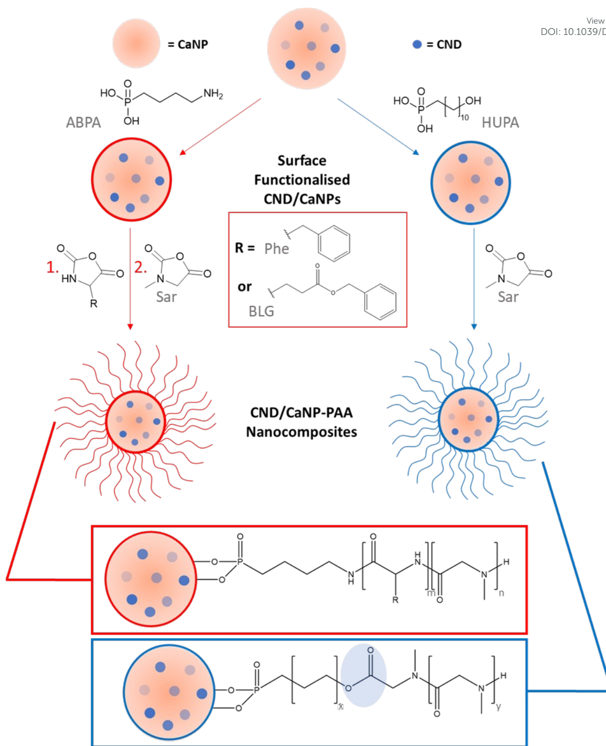
Scheme 1. (a) The creation of amino and hydroxyl-functionalised CaNPs that contain CNDs, followed by ROP to yield the nanocomposites CND/CaNP-APBA-PPhe- b -PSar or CND/CaNP-APBA-PBLG- b -PSar (left) and CND/CaNP-HUPA-PSar (right). The ester link that renders CND/CaNP-HUPA-PSar 82 susceptible to acid-catalysed hydrolysis is highlighted.
