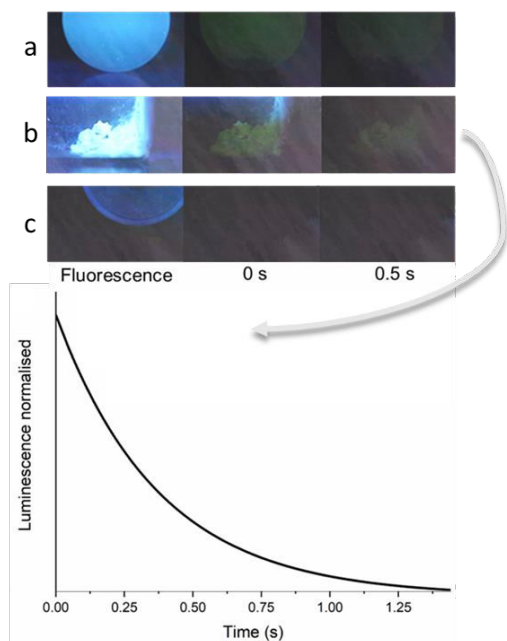
Fig. 5. Images determining the presence of afterglow of (a) CND/CaNP-ABPA-PPhe 4 -b-PSar 16 in pH 7.4 PBS buffer solution, (b) CND/CaNP-ABPA-PPhe 4 -b-PSar 16 following removal from solution and drying, (c) CND/CaNP-ABPA-PPhe 4 -b-PSar 16 suspended in pH 5 acetate buffer solution. The normalised afterglow lifetime of CND/CaNP-ABPA-PPhe 4 -b-PSar 16 following removal from solution is presented below the microscopy images. Afterglow was triggered by irradiating the samples with UV light at 365 nm for a few seconds beforehand.
