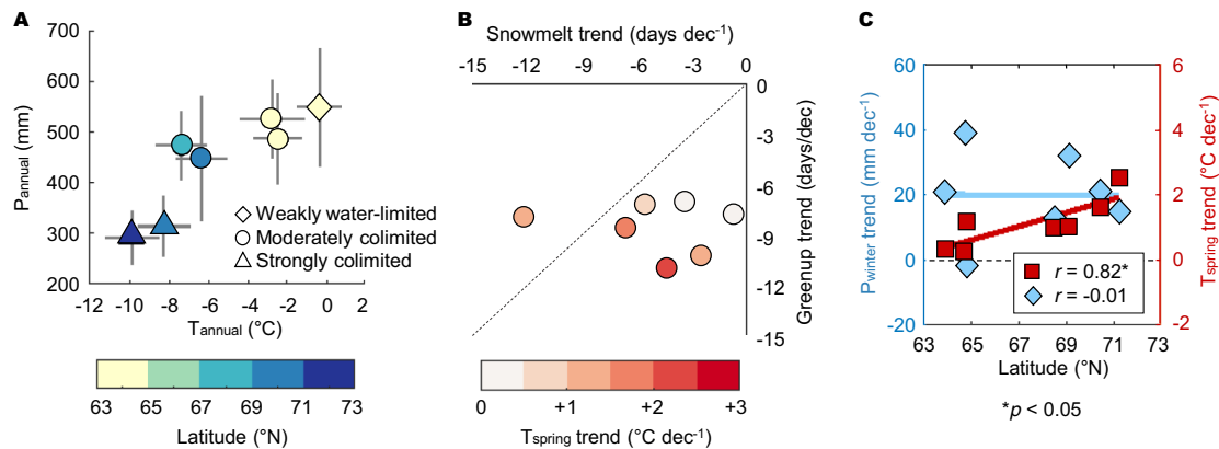
Fig. 2 Latitudinal gradients in climatic conditions and greenup and snowmelt timings. A Annual mean temperature ( T_{annual} ) and annual total precipitation ( P_{annual} ) at each site (2001–2018 means in symbols and one std. dev. in lines) with latitude (in color) and climatic limits (see Methods—Study sites). B Long-term trends of snowmelt and greenup timings at each site (in circles, Fig. S3) and the spring mean temperature trend ( T_{spring} , Apr.–Jun., in color). C Correlations of long-term trends of T_{spring} and winter precipitation ( P_{winter} , Jan.–May) with latitude.
