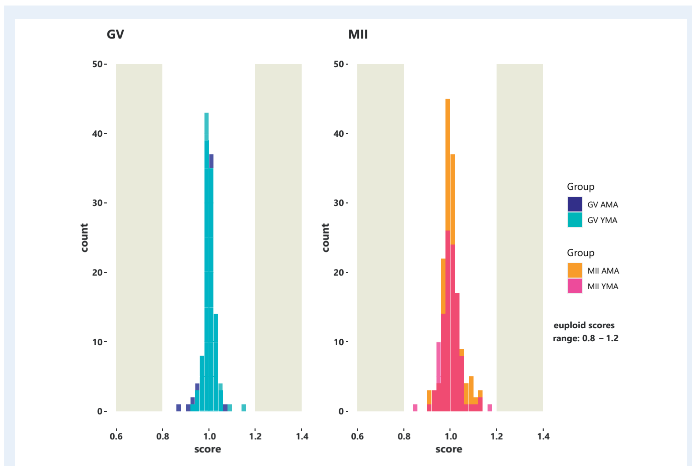
Figure 1. Bell shaped histograms illustrate the score of the average euploid GV and MII oocytes. Normal scores generated by scploidy software range between 0.8 and 1.2 (euploidy status). Based on the allele specific gene expression, a score of 1 indicates that no aneuploid chromosomes were present. The results derived from the RNA sequencing data analysis. AMA, advanced maternal age; GV oocyte, germinal vesicle oocyte; MII oocyte, metaphase II oocyte; YMA, young maternal age.
